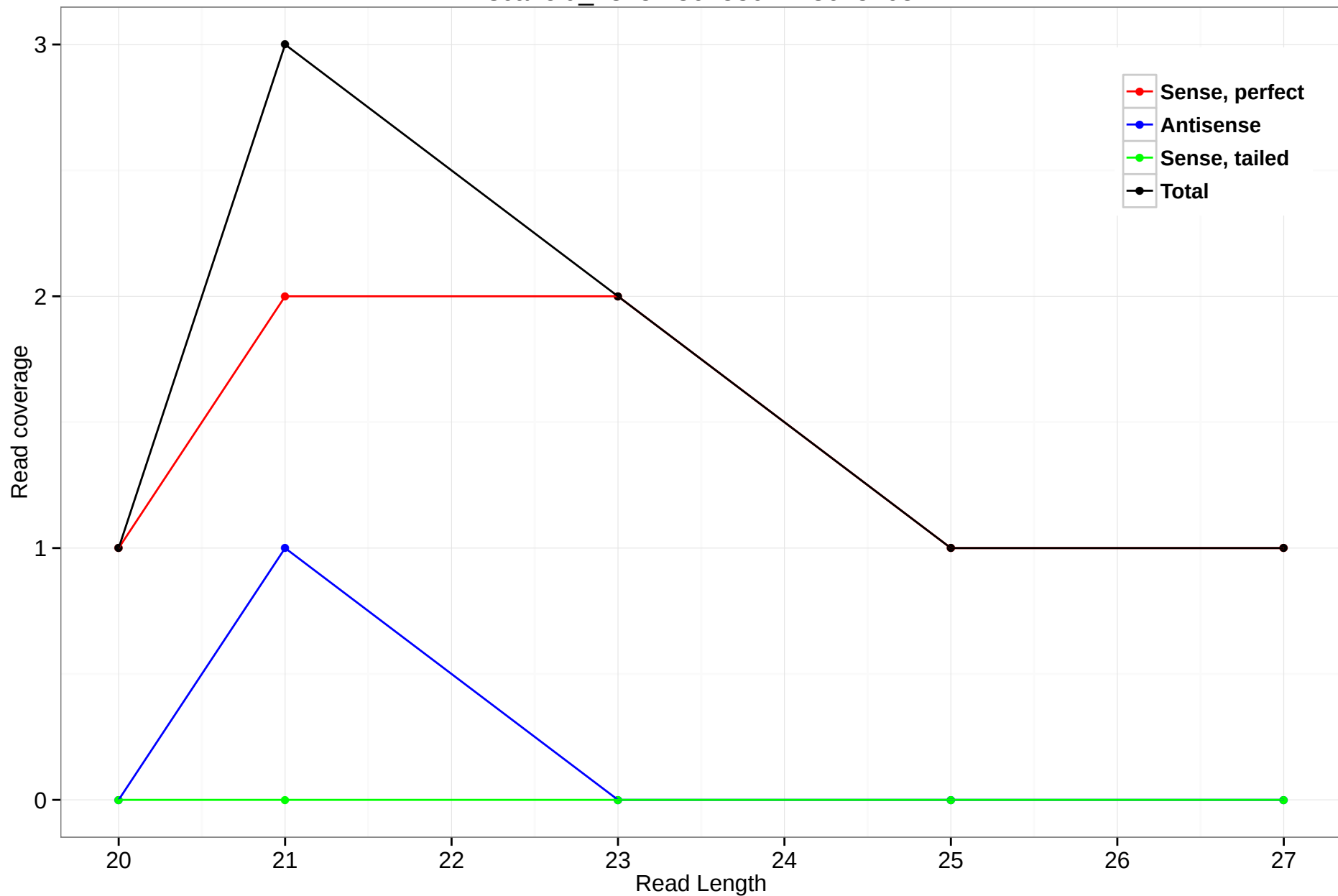
scaffold_4845:18615304-18615705
