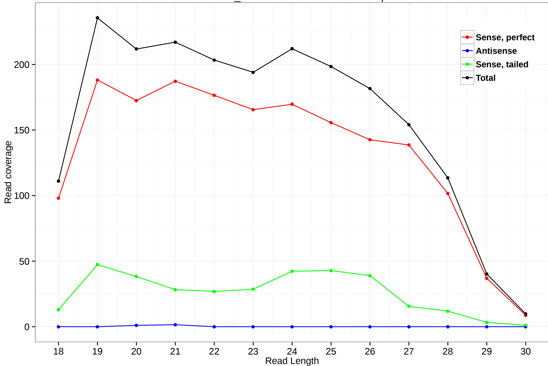
scaffold_4845:18559285-18560339.3p
