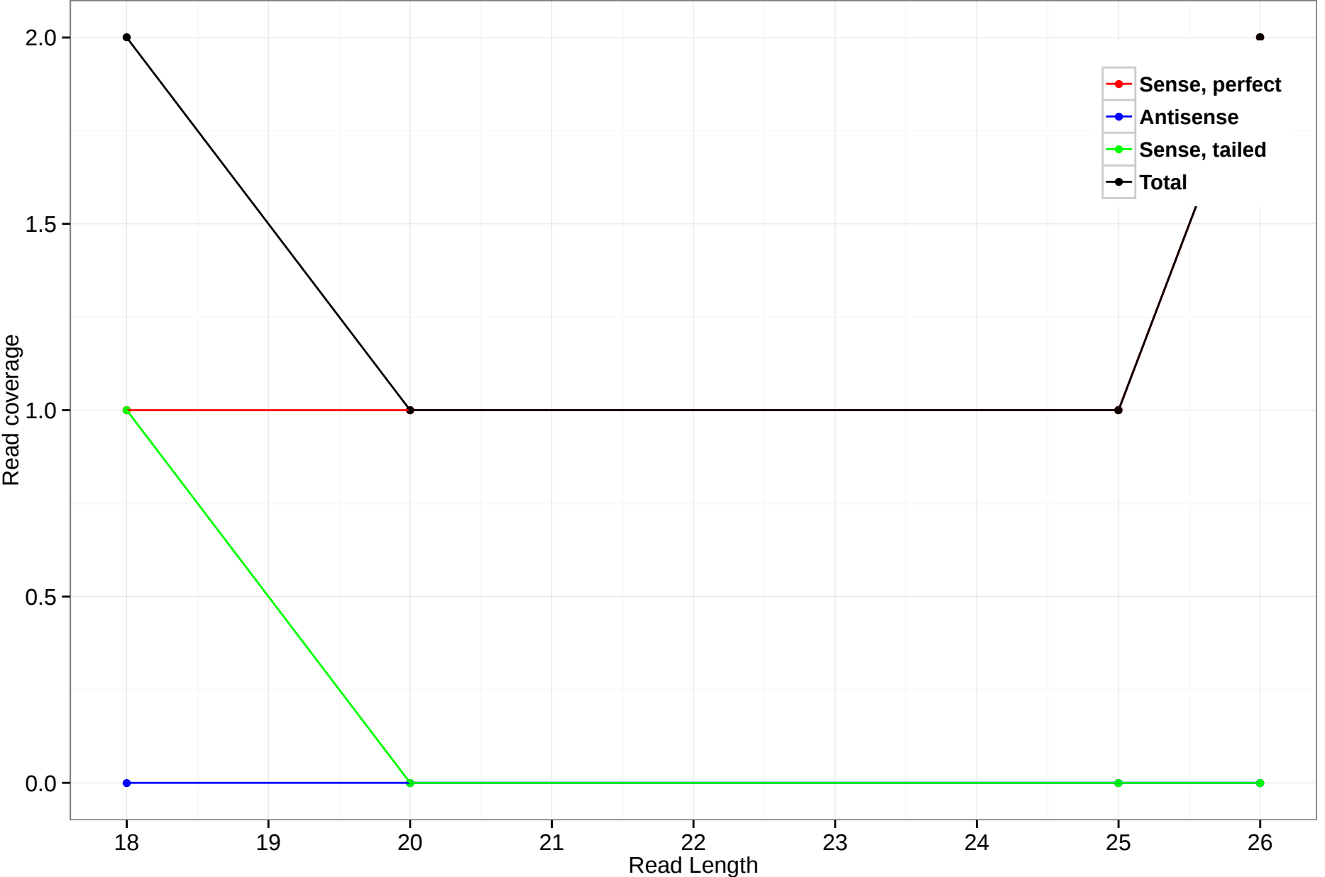
scaffold_4845:18458394-18459001.5p
