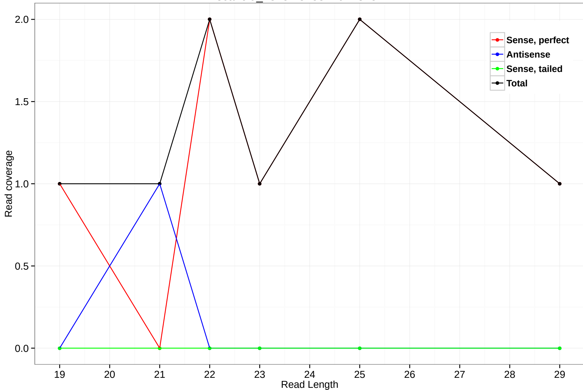
scaffold_4845:18183720-18184177
