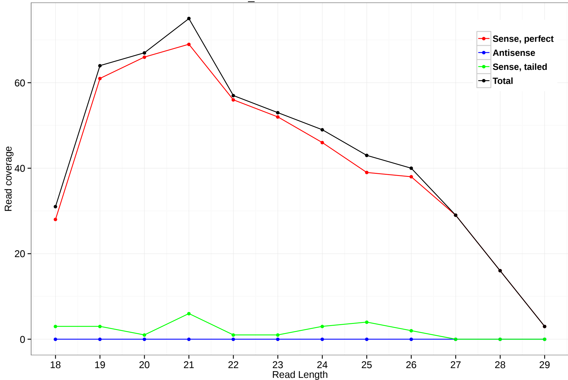
scaffold_4845:18012787-18012946
