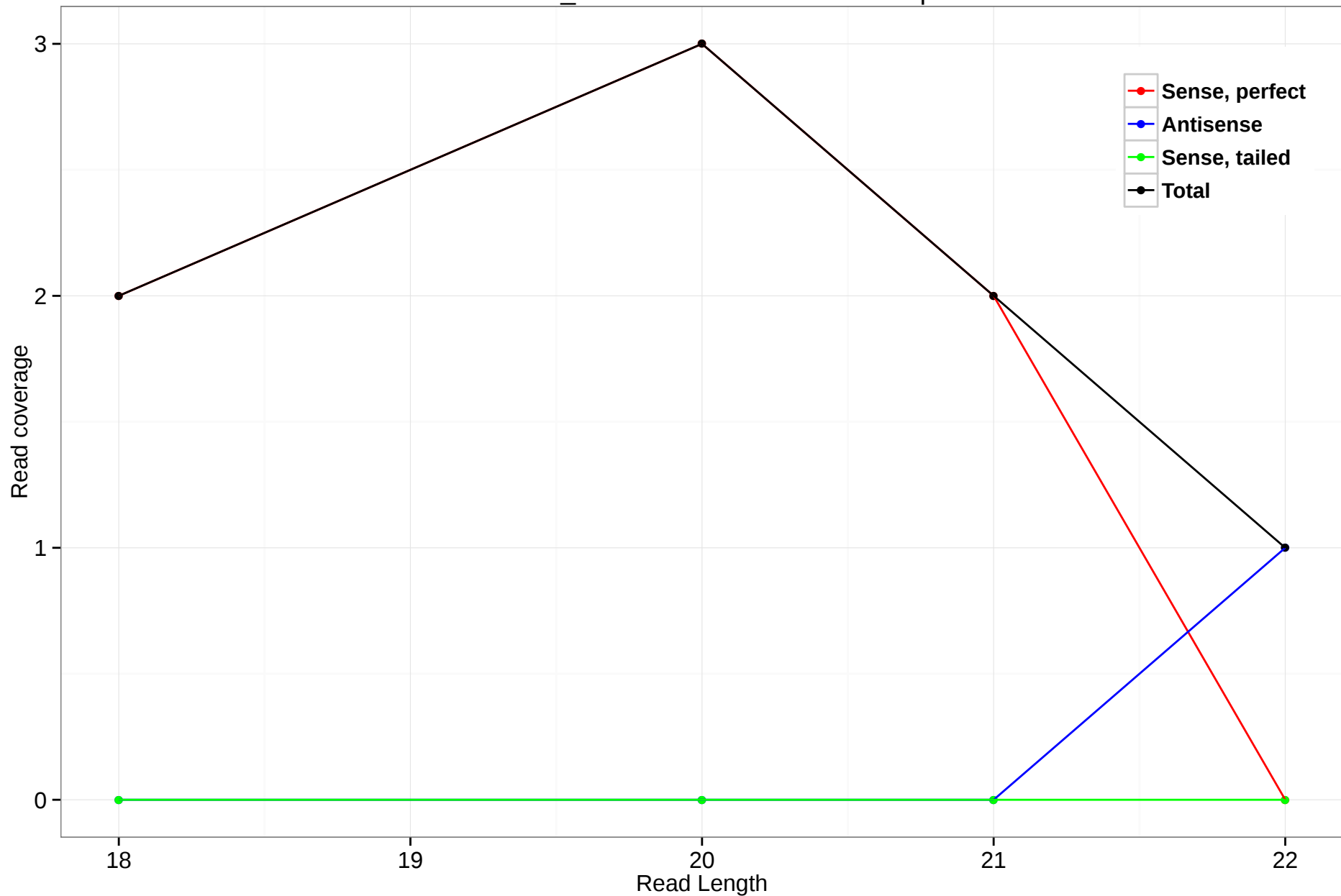
scaffold_4845:17957745-17967779.5p
