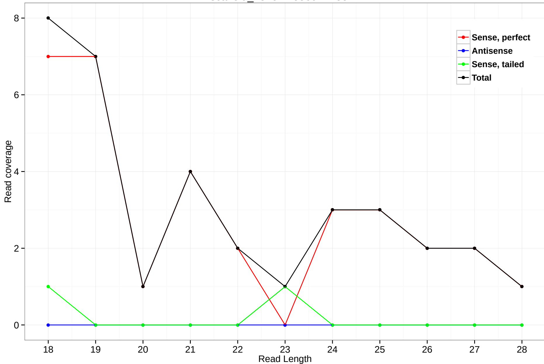
scaffold_4845:175569-175841
