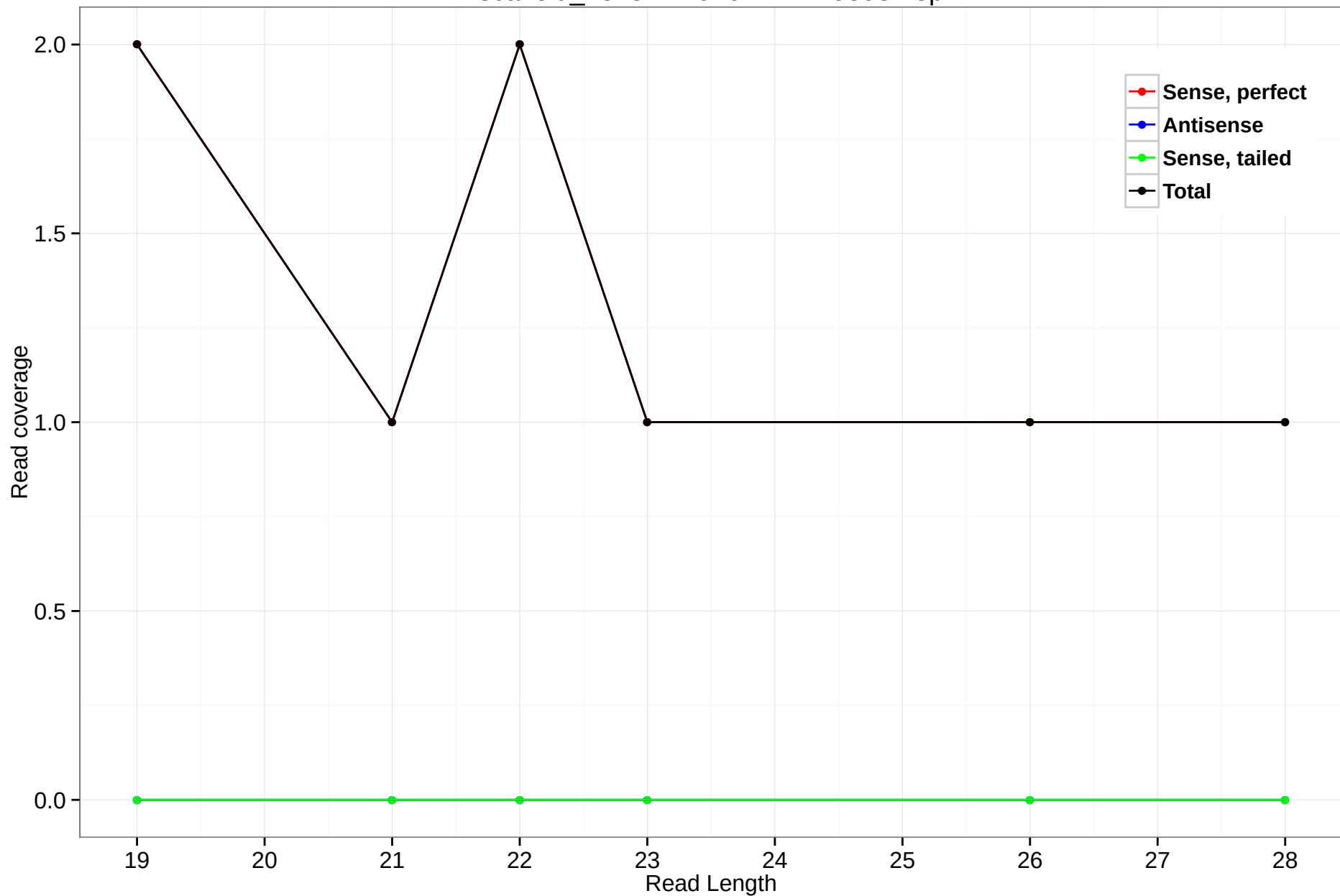
scaffold_4845:17297611-17298984.3p
