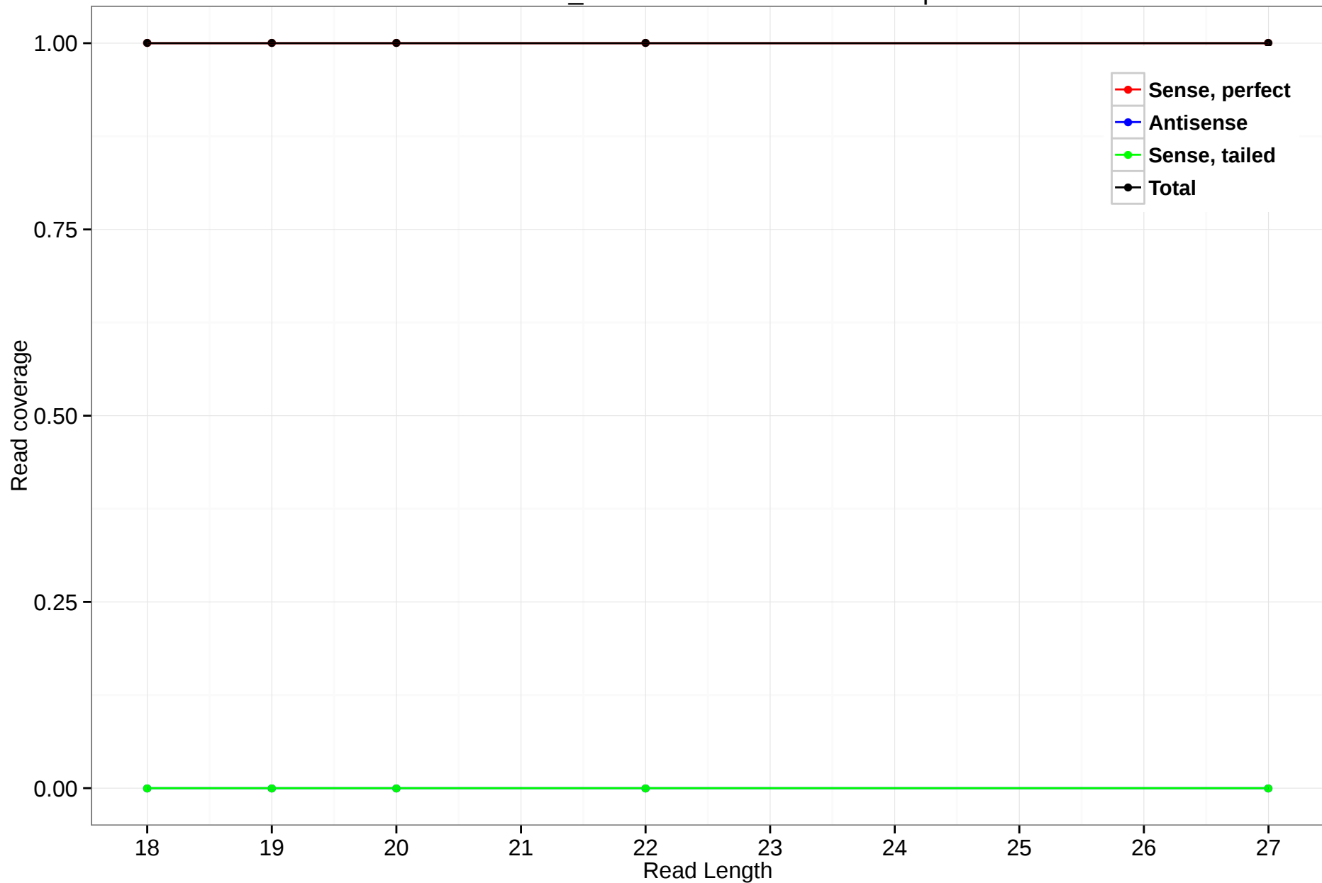
scaffold_4845:16766879-16768240.3p
