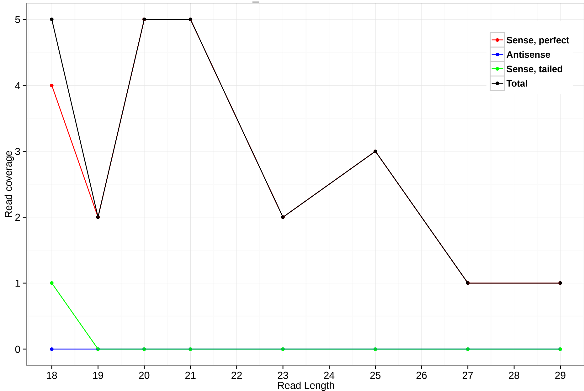
scaffold_4845:16680712-16680876
