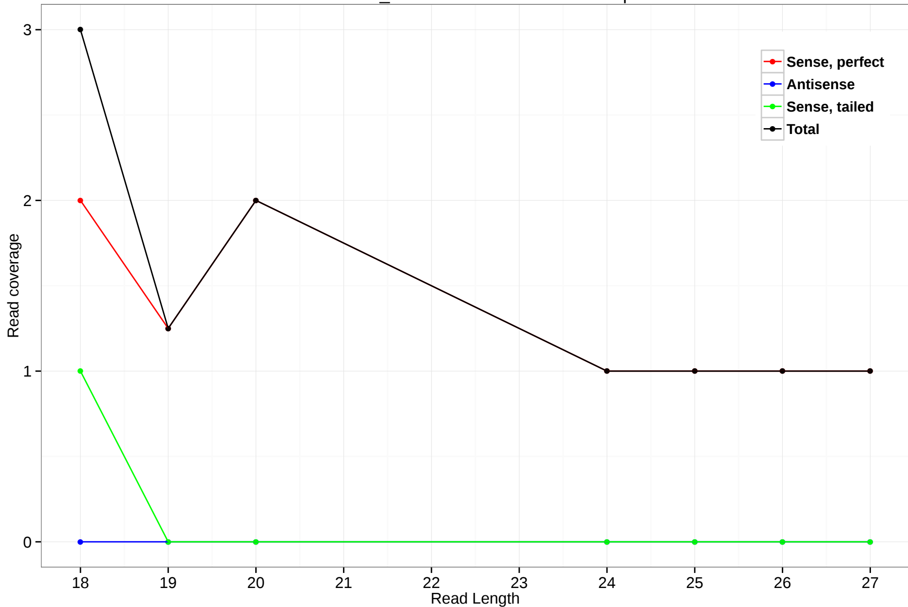
scaffold_4845:16008648-16011985.5p
