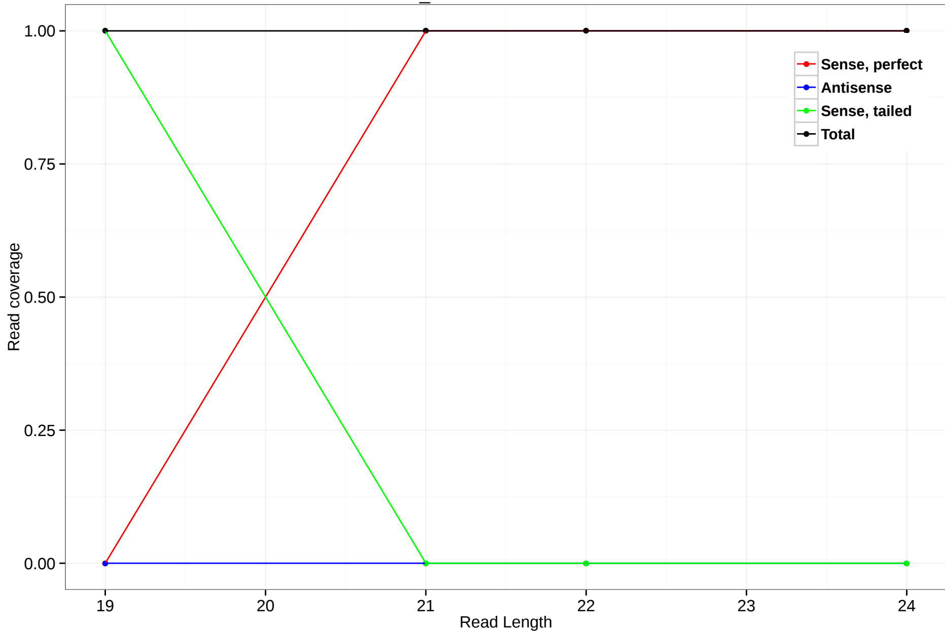
scaffold_4845:15801170-15801324
