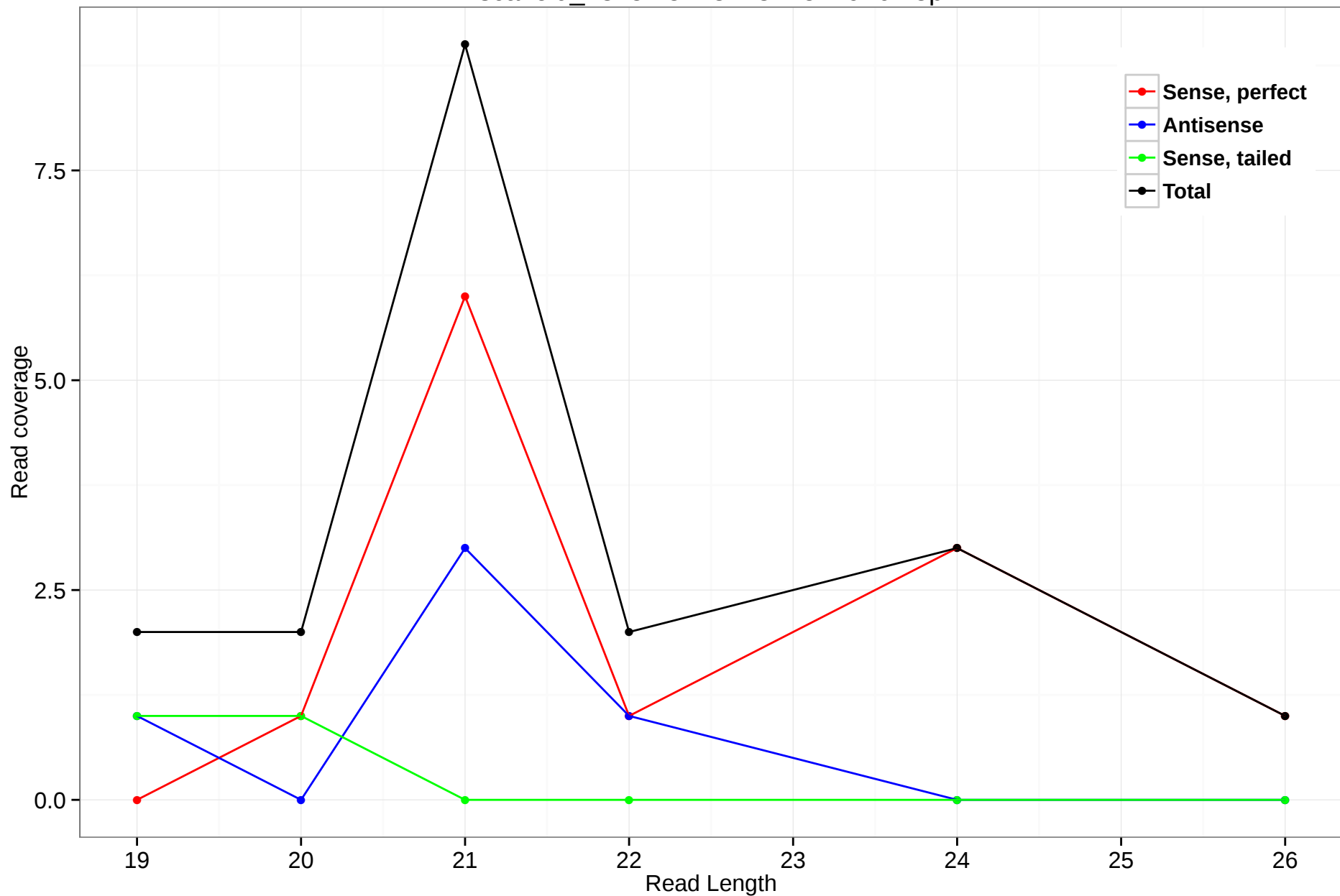
scaffold_4845:15778118-15779764.5p
