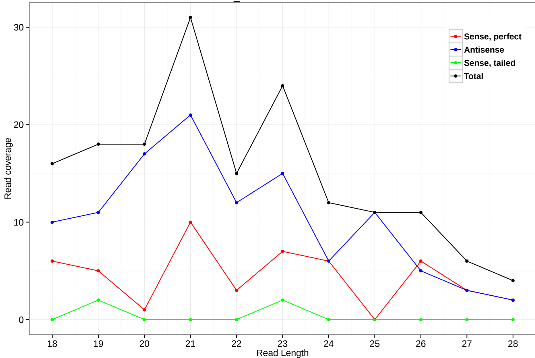
scaffold_4845:15701131-15701683
