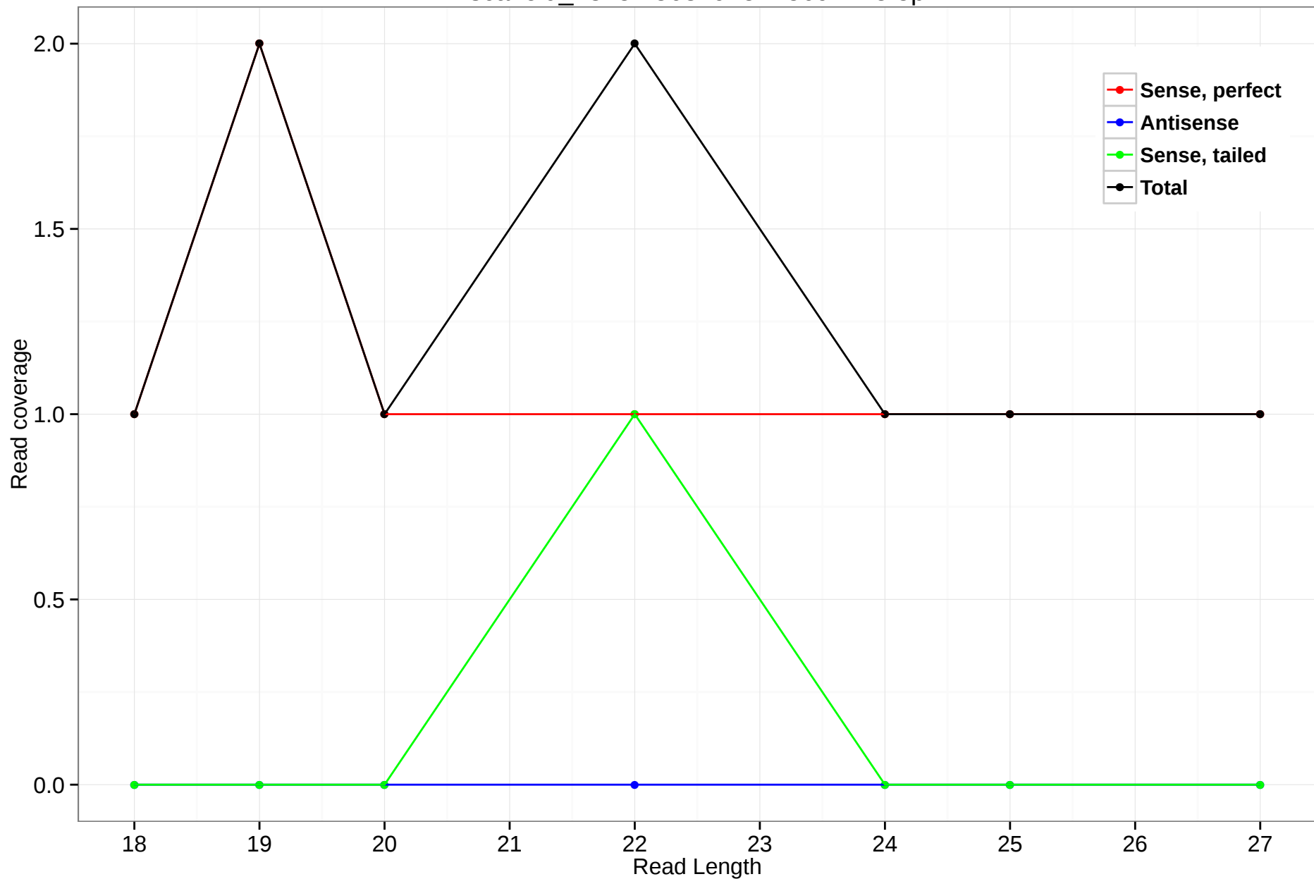
scaffold_4845:15687945-15691775.5p
