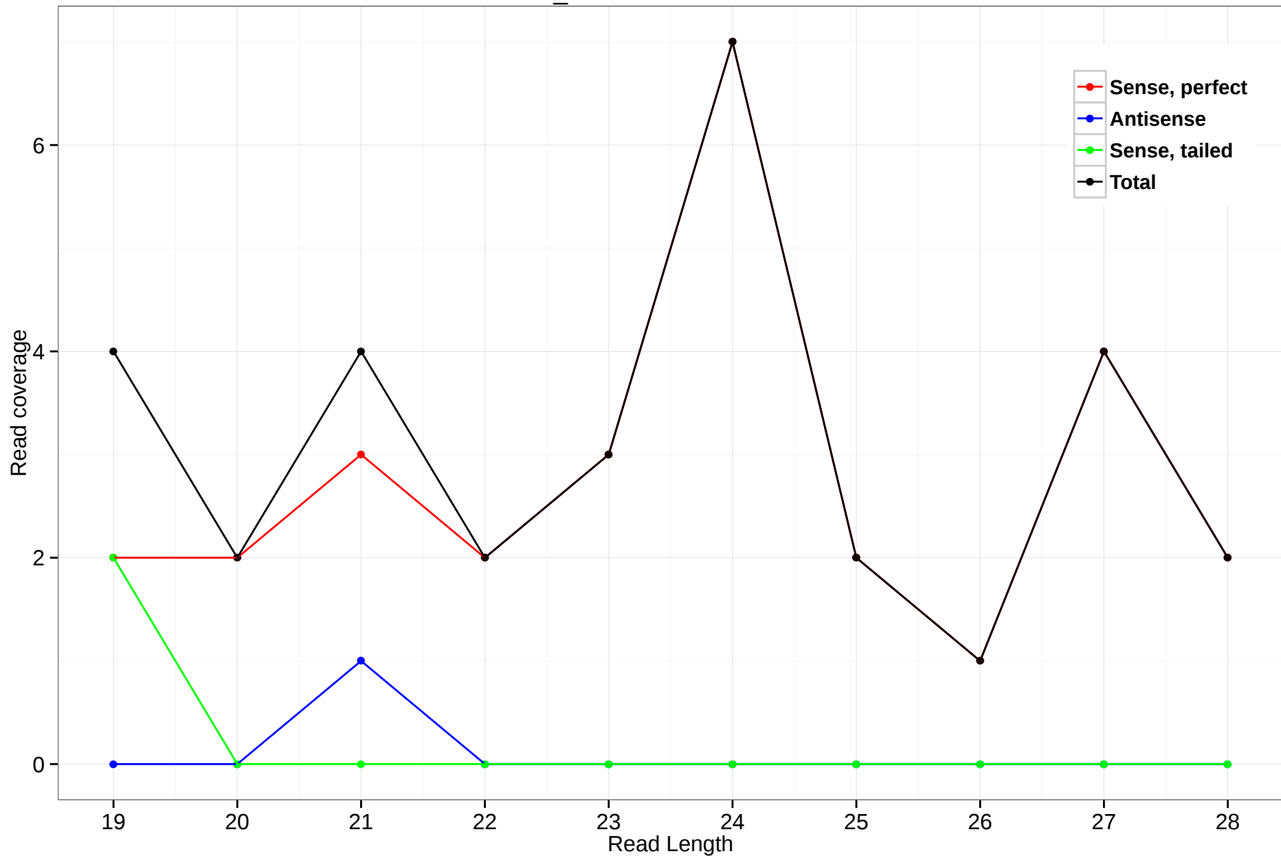
scaffold_4845:15363268-15363644
