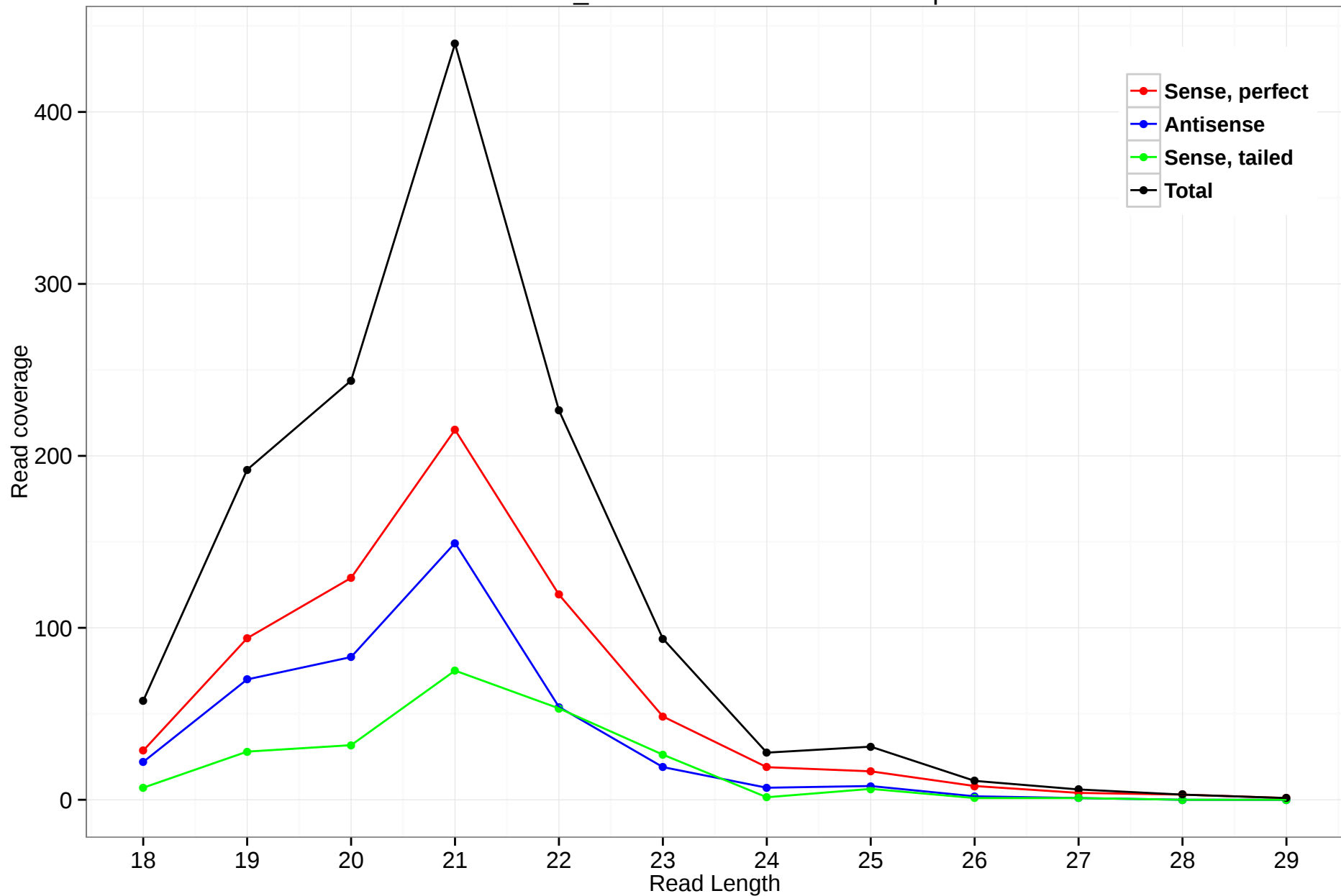
scaffold_4845:15341417-15342188.3p
