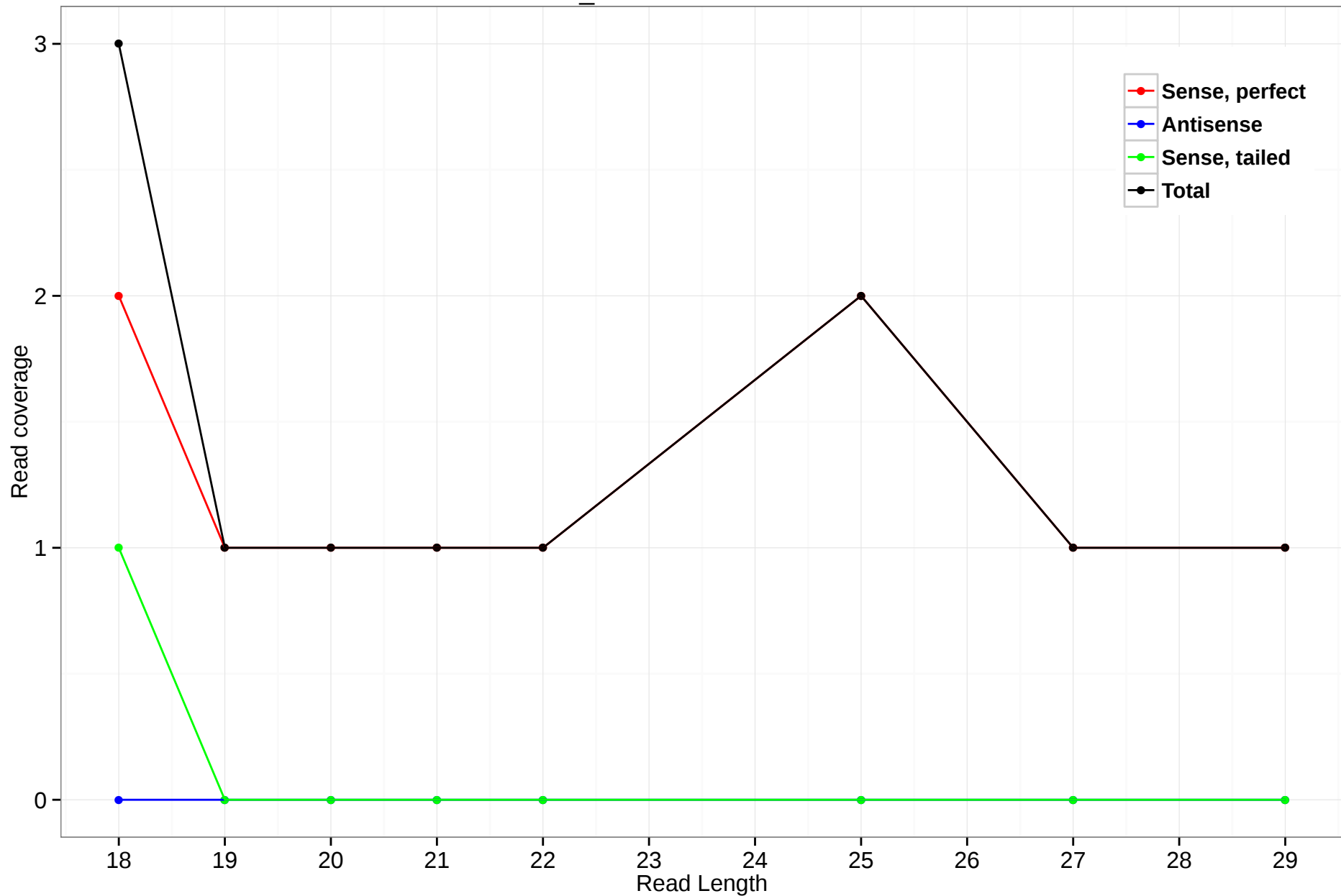
scaffold_4845:15002318-15002807
