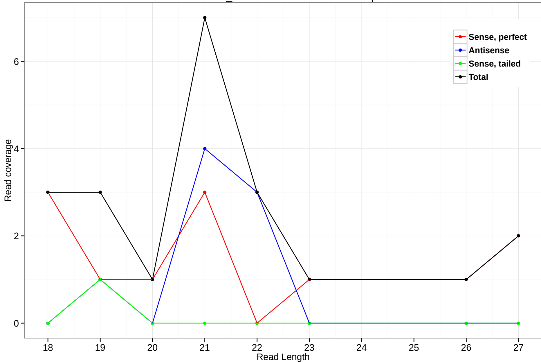
scaffold_4845:14637492-14639011.3p
