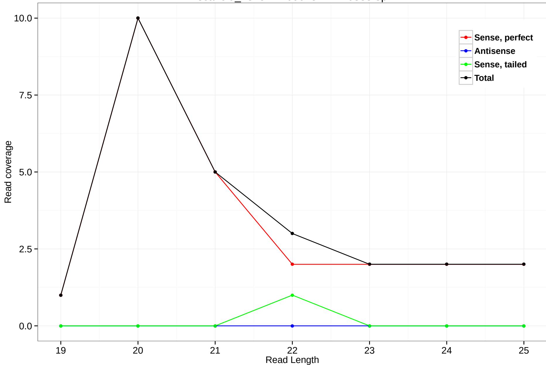
scaffold_4845:14109028-14110388.3p
