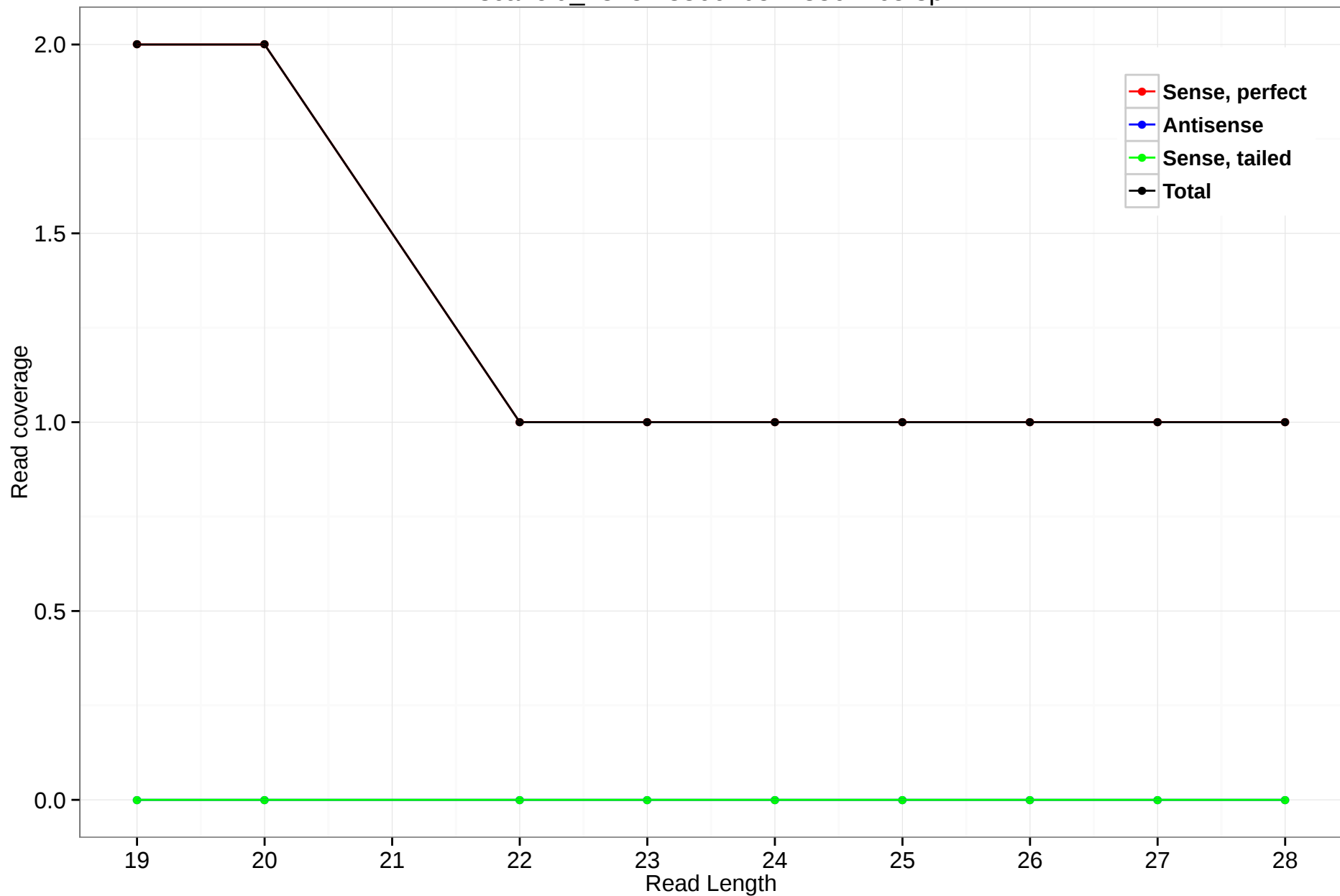
scaffold_4845:13866405-13867165.3p
