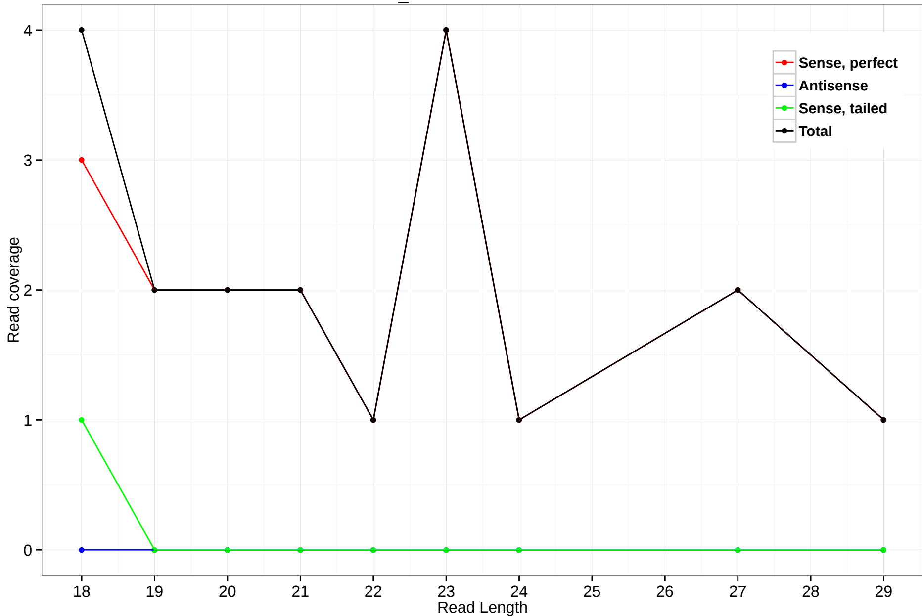
scaffold_4845:13831562-13831954
