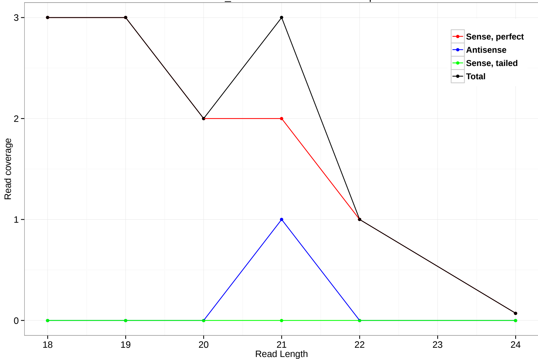
scaffold_4845:12538963-12540989.5p
