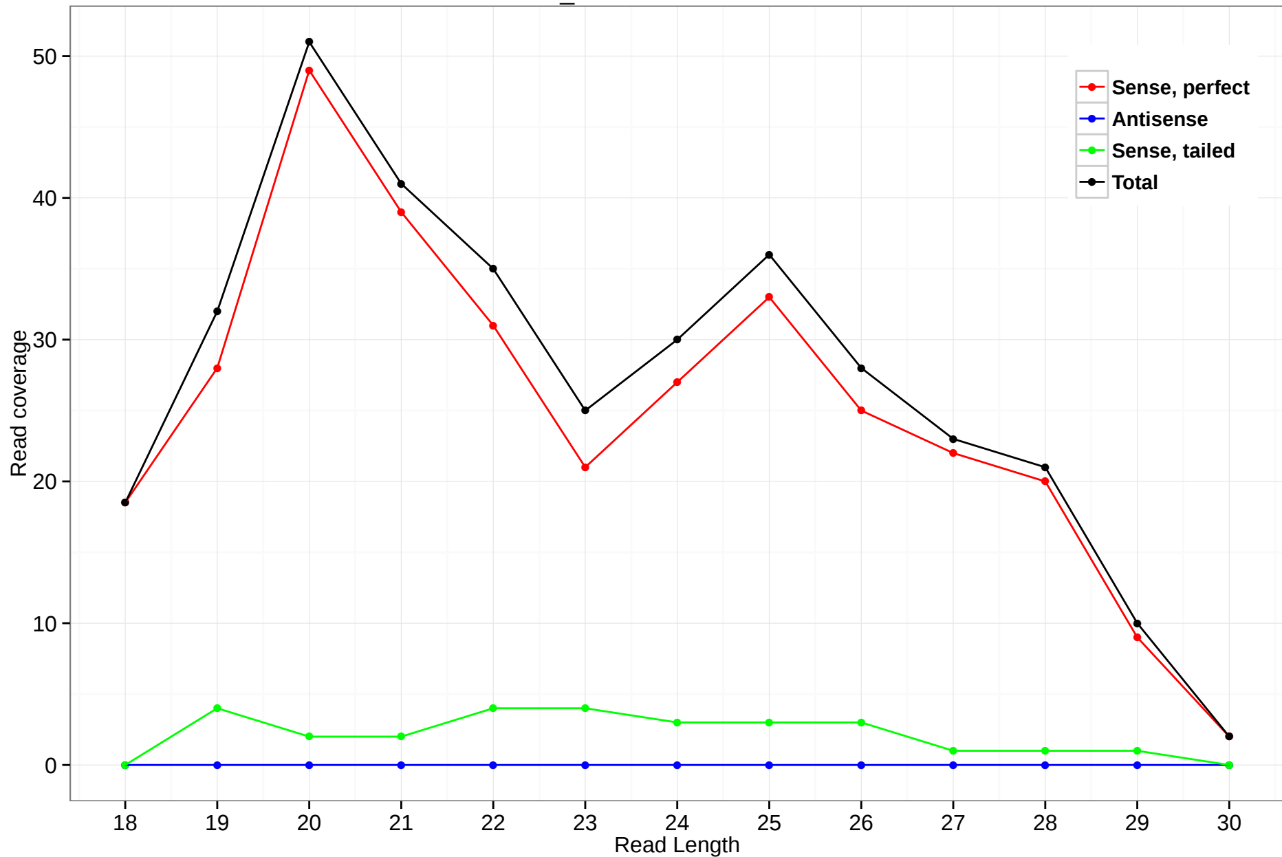
scaffold_4845:11356431-11356744
