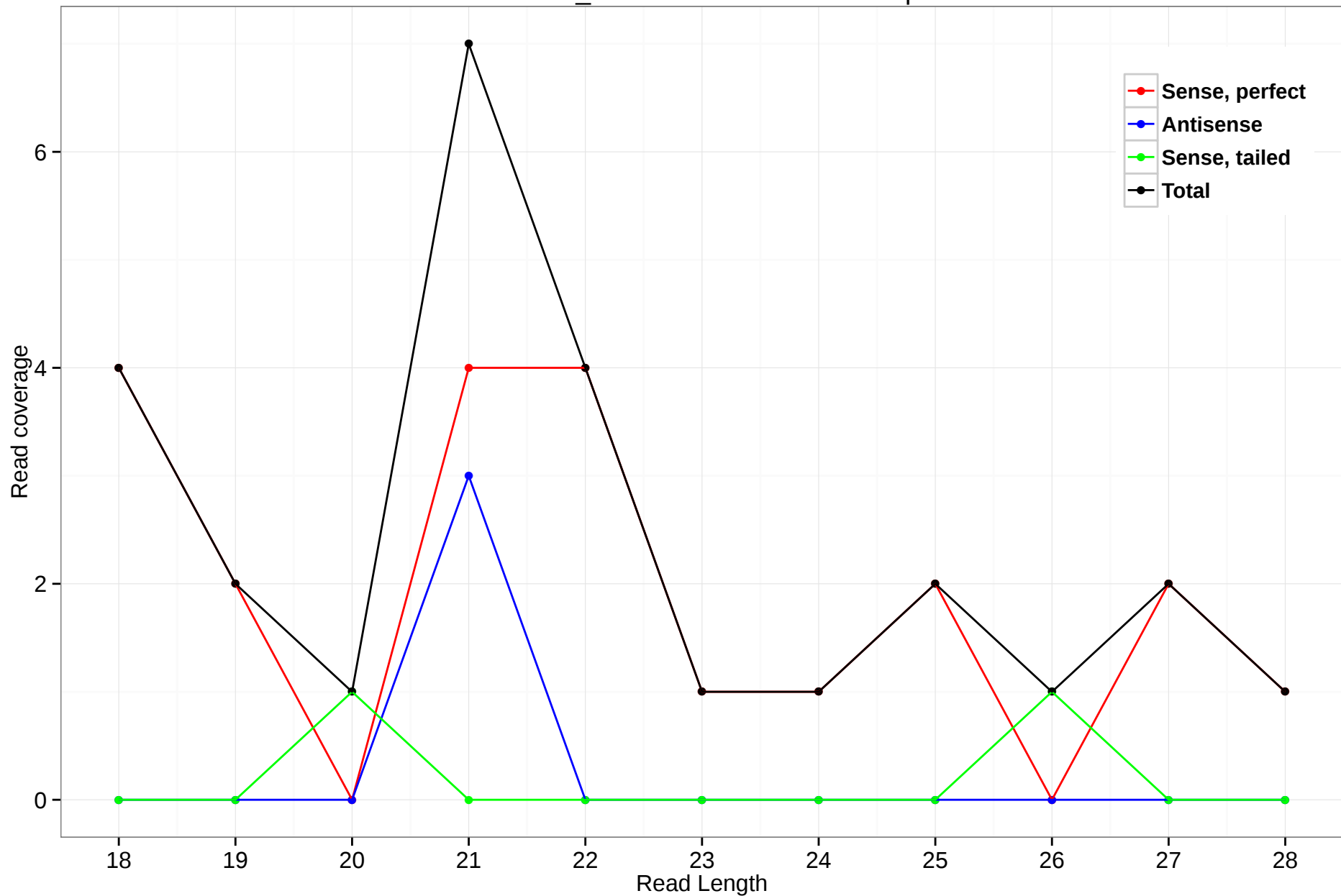
scaffold_4820:9894187-9895053.5p
