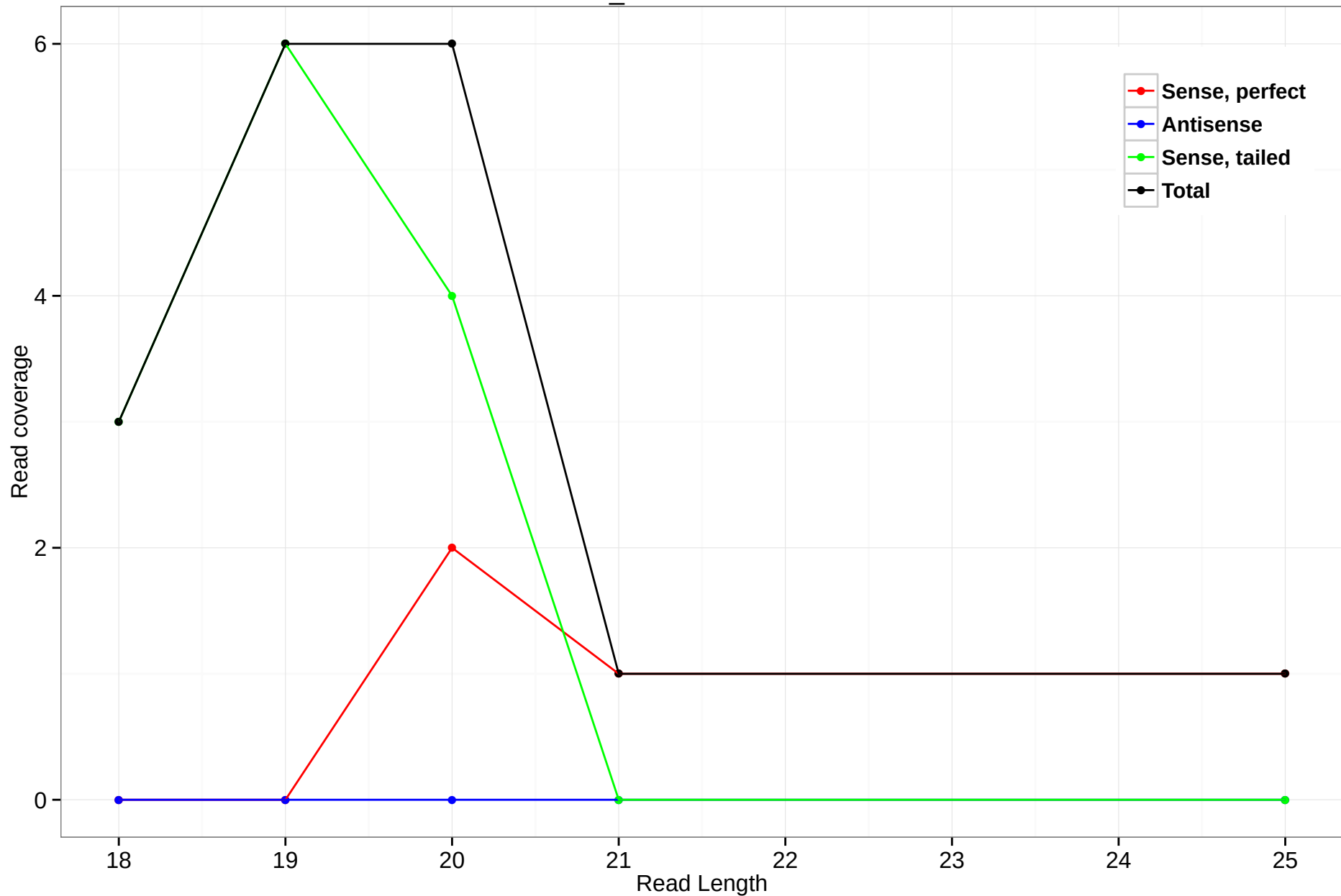
scaffold_4820:980298-980768
