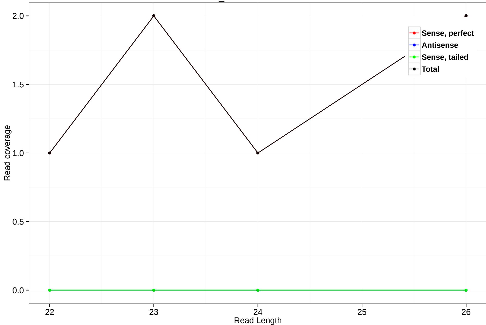
scaffold_4820:9760346-9760509
