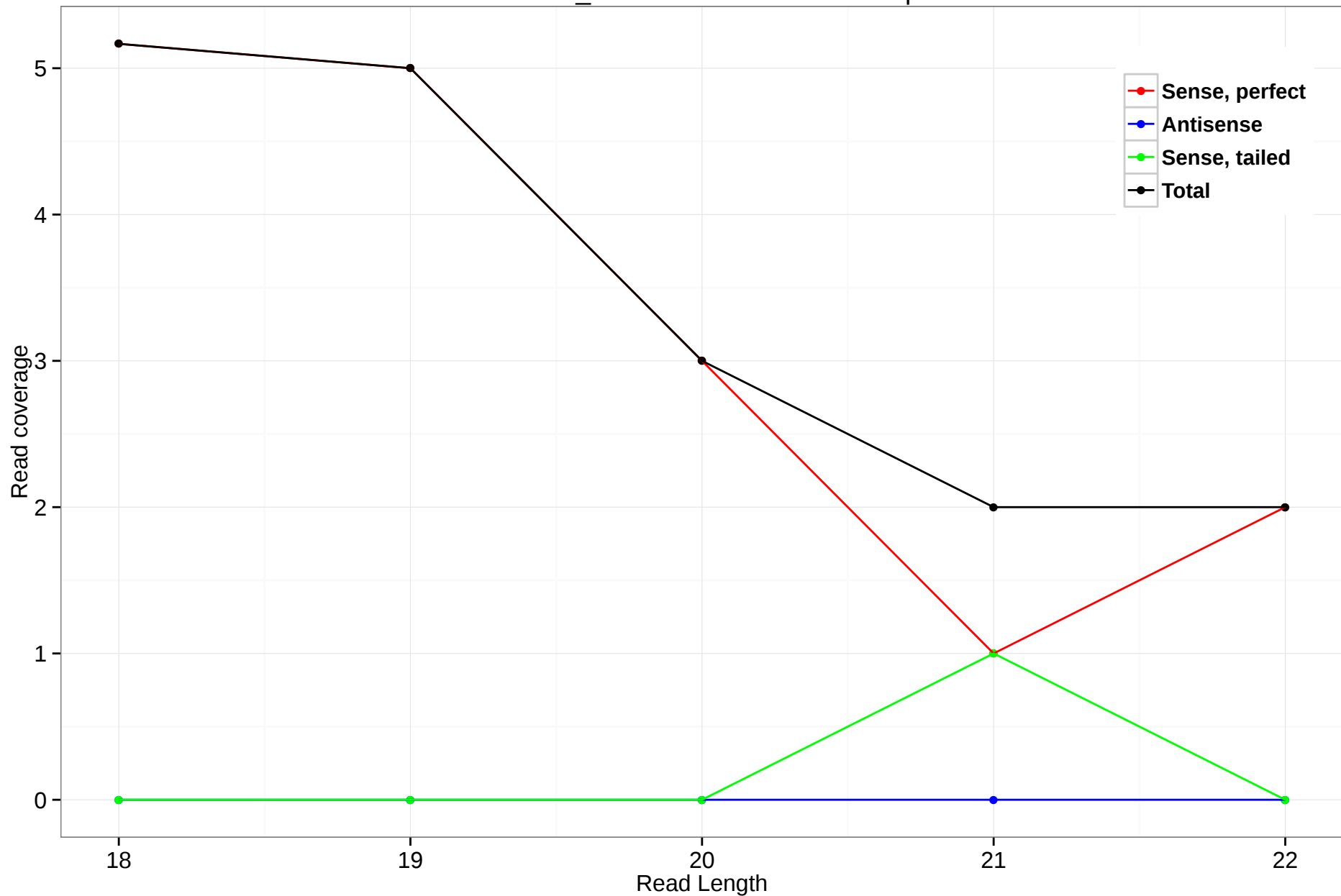
scaffold_4820:9482126-9493567.5p
