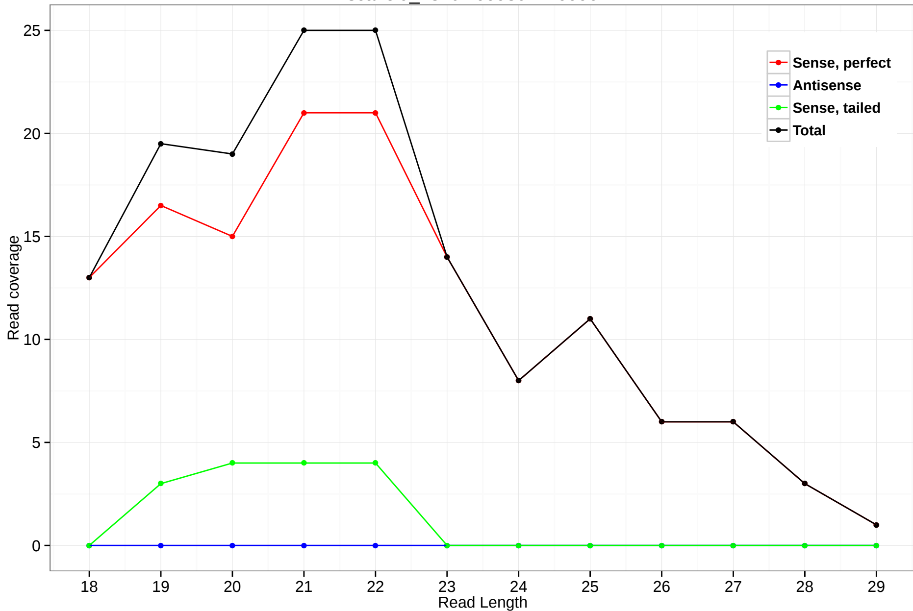
scaffold_4820:7999304-7999671
