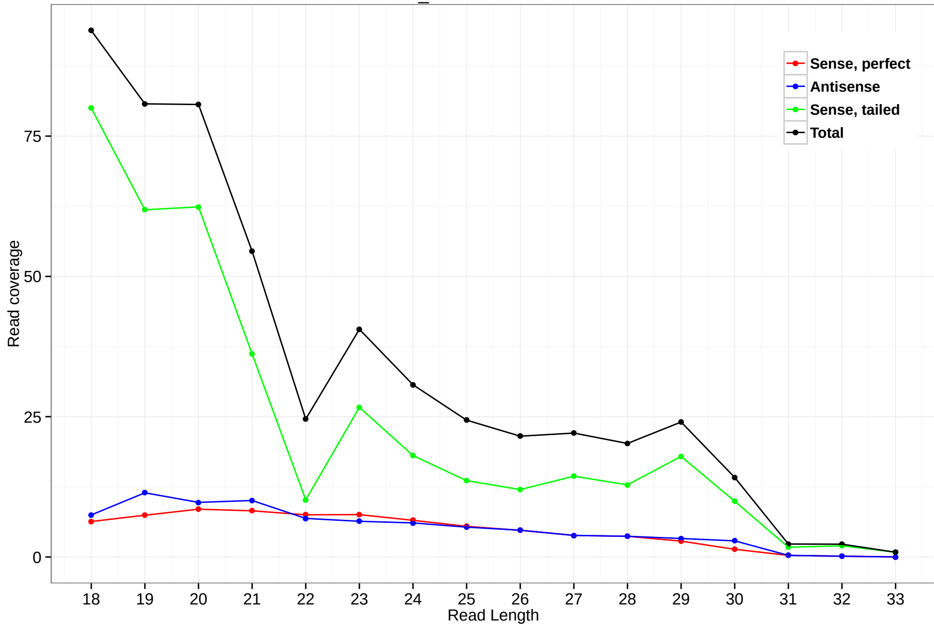
scaffold_4820:7308632-7309155
