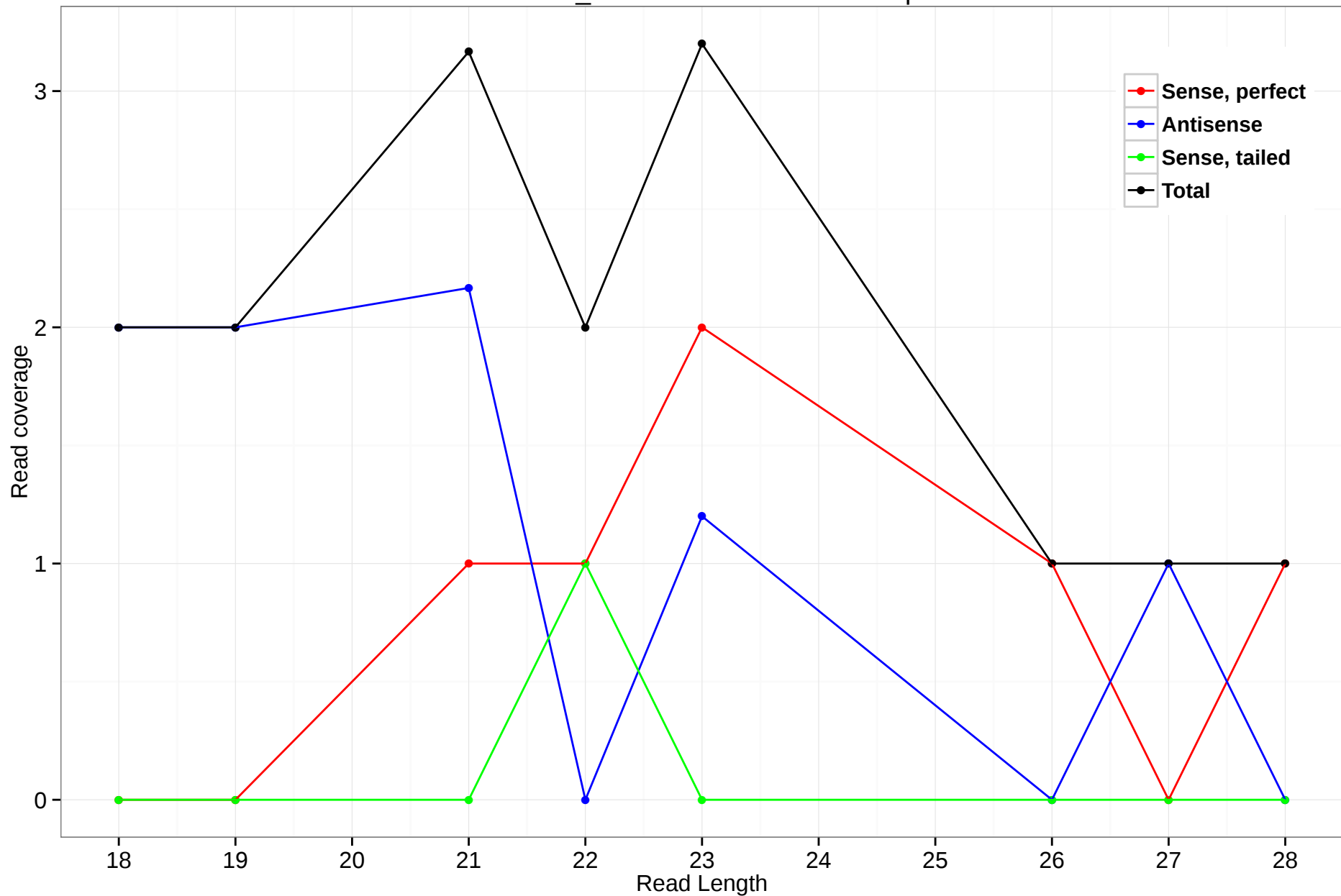
scaffold_4820:7176319-7177107.5p
