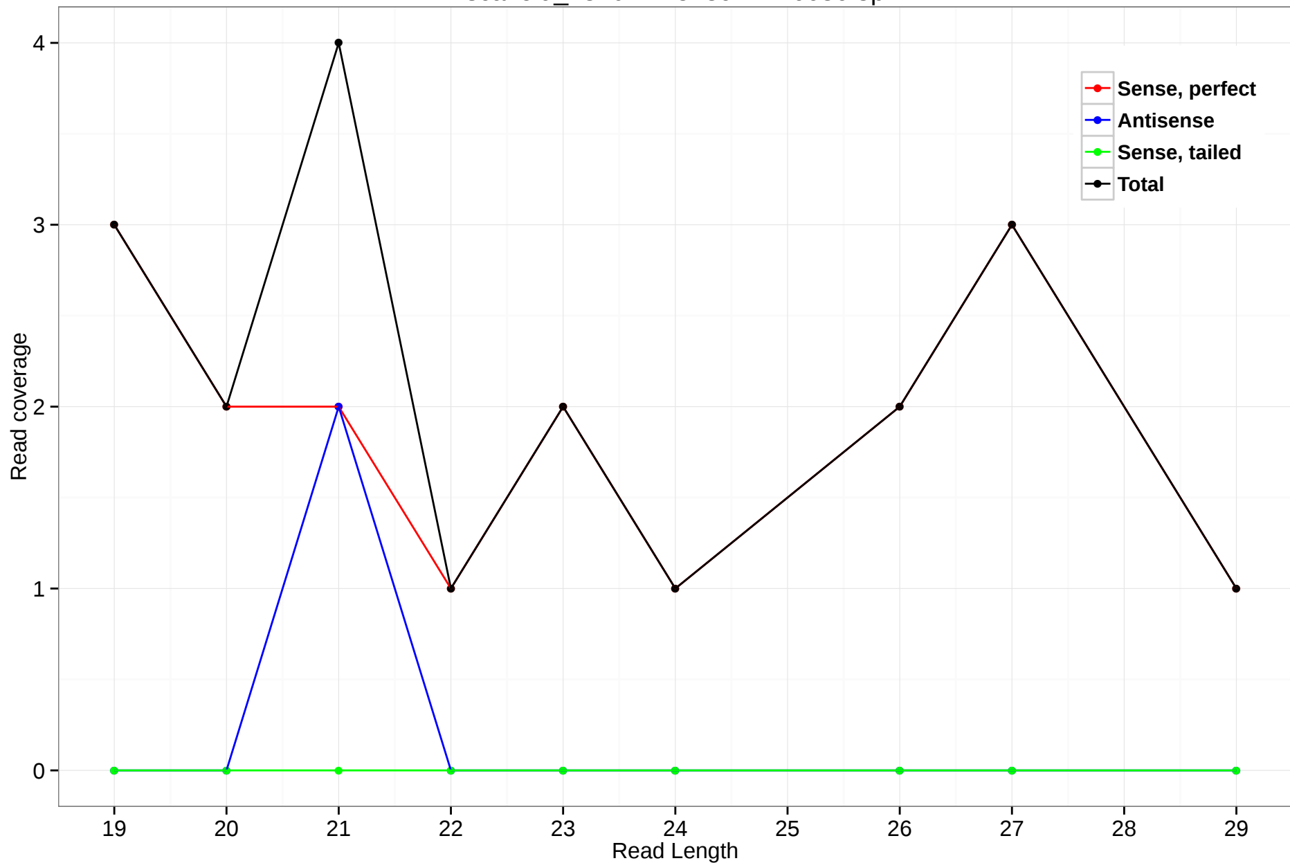
scaffold_4820:7175789-7176686.3p
