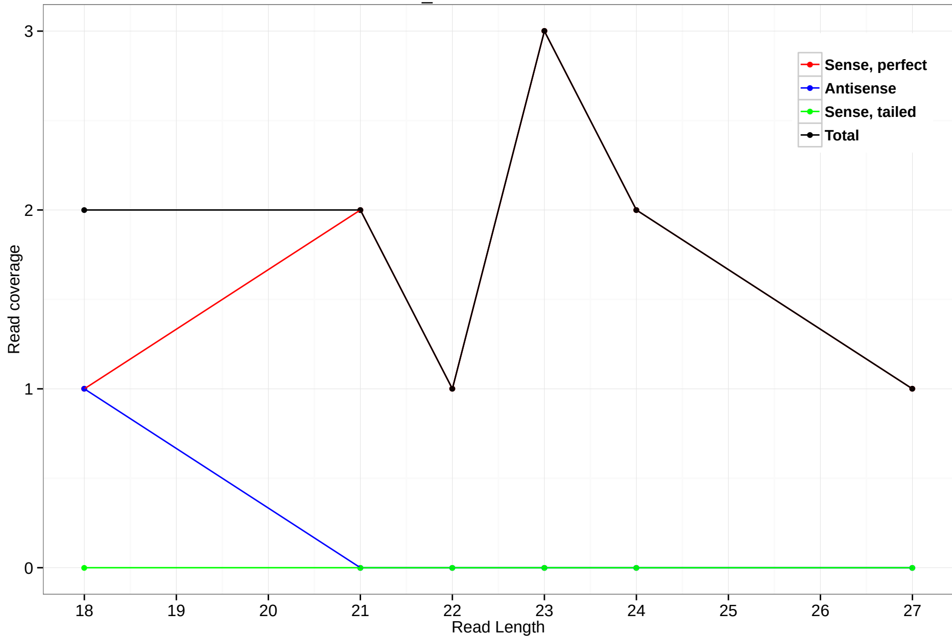
scaffold_4820:6994735-6995162
