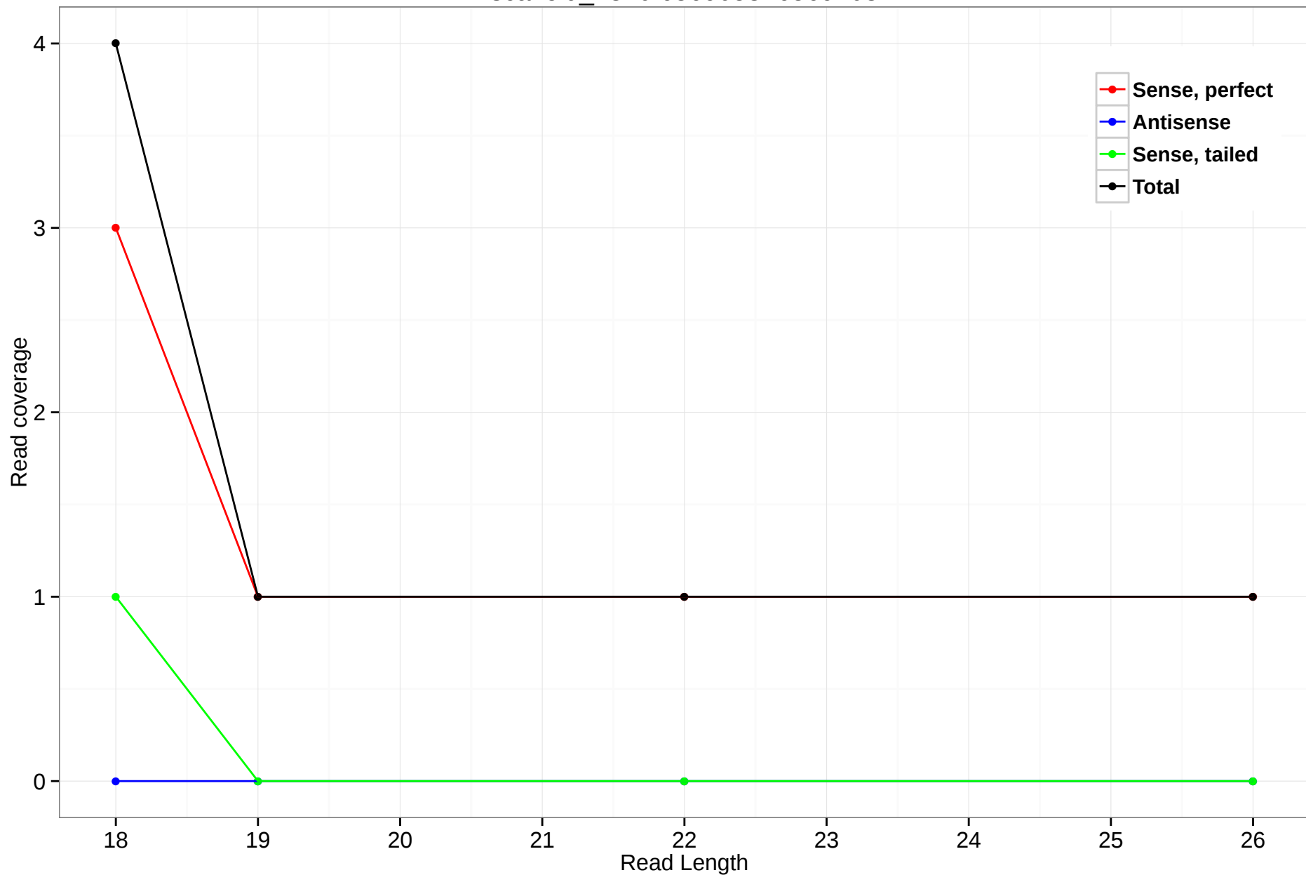
scaffold_4820:6569053-6569403
