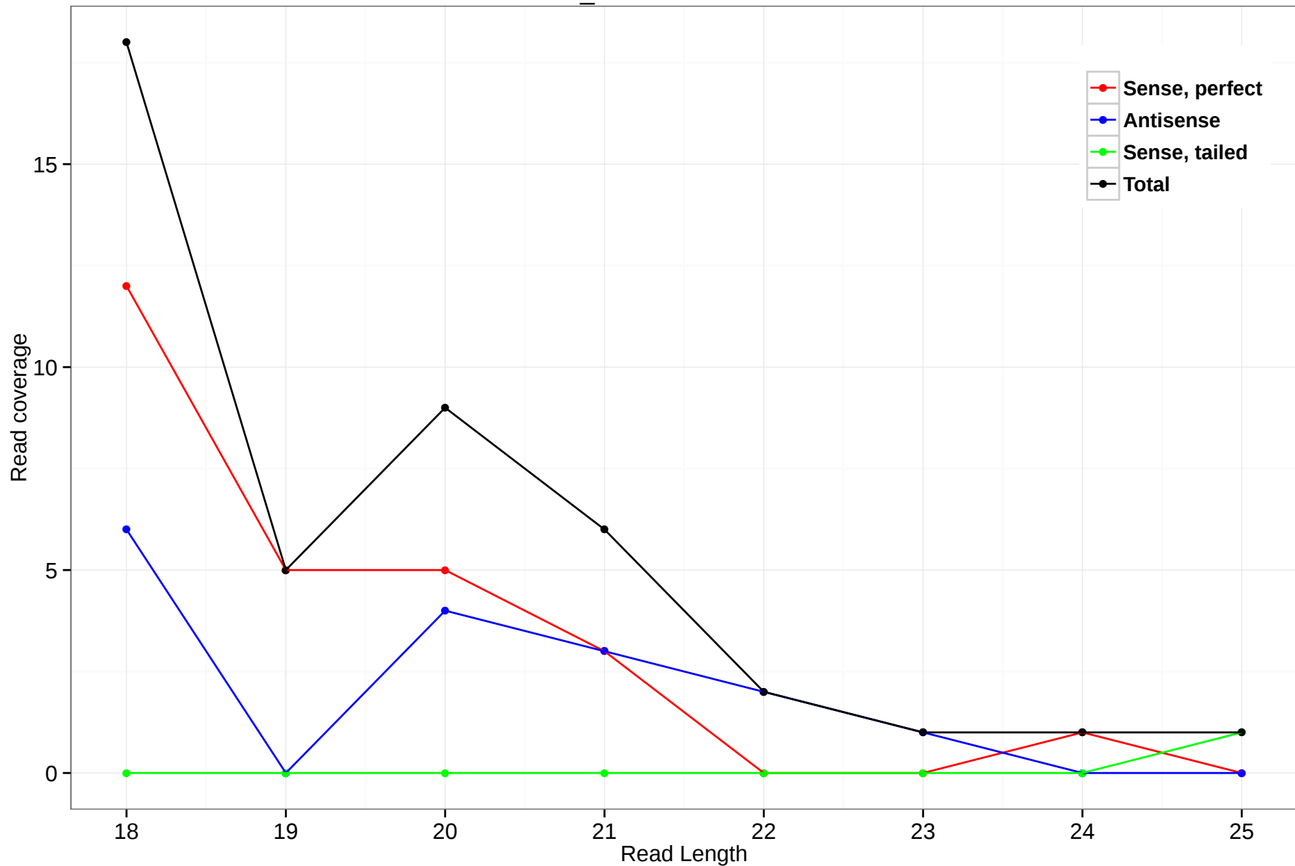
scaffold_4820:6430938-6431173
