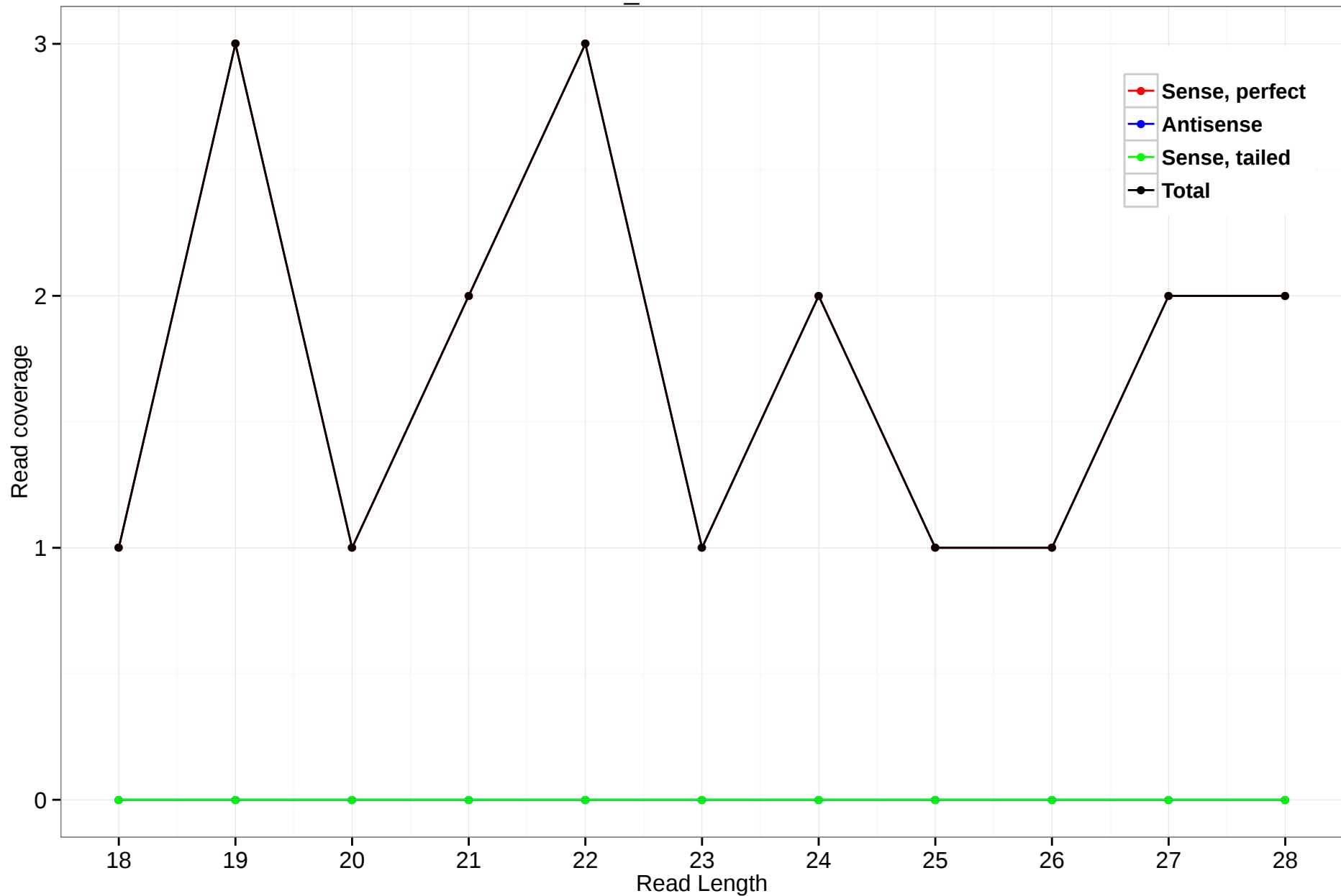
scaffold_4820:59820-60094
