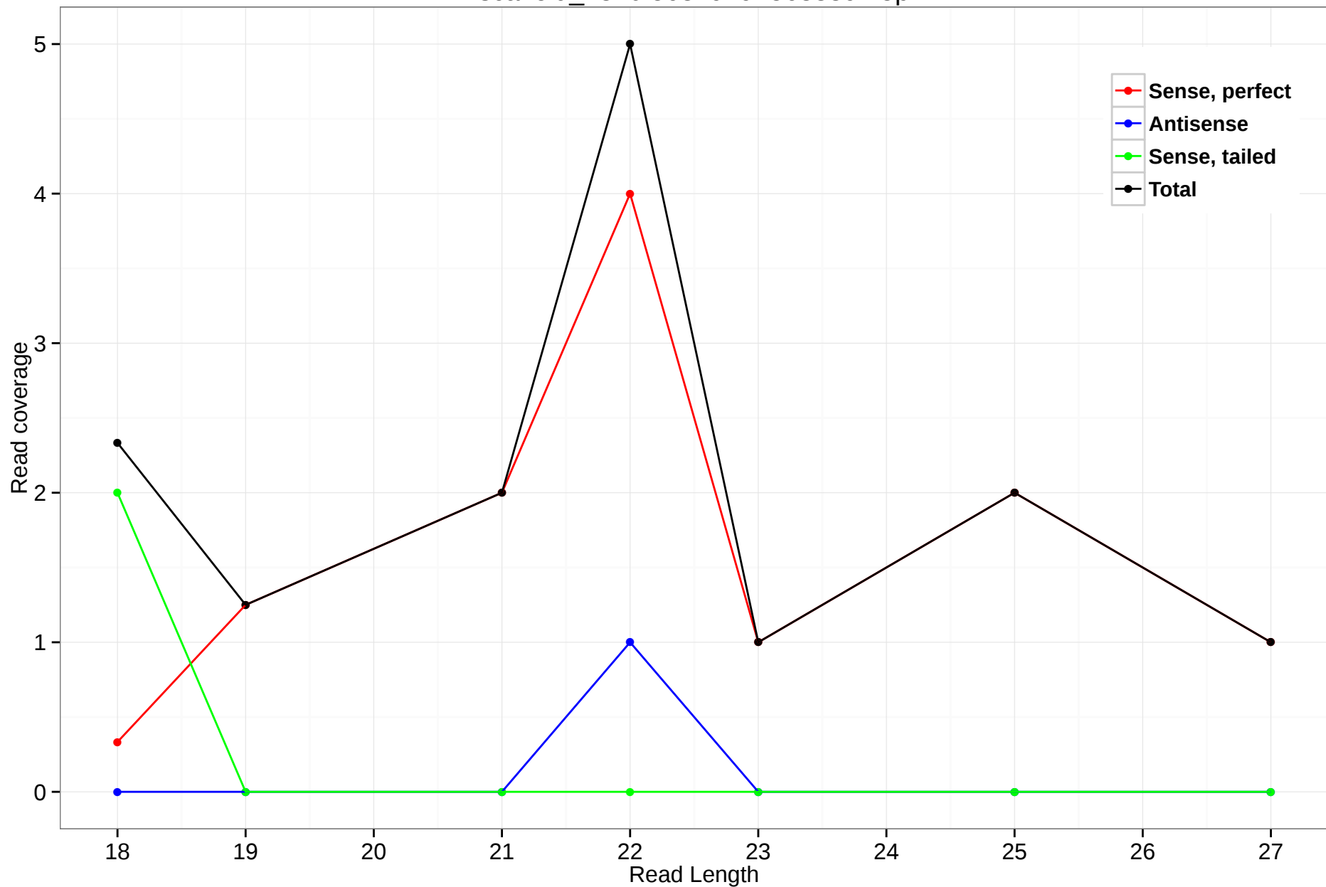
scaffold_4820:5687929-5688897.5p
