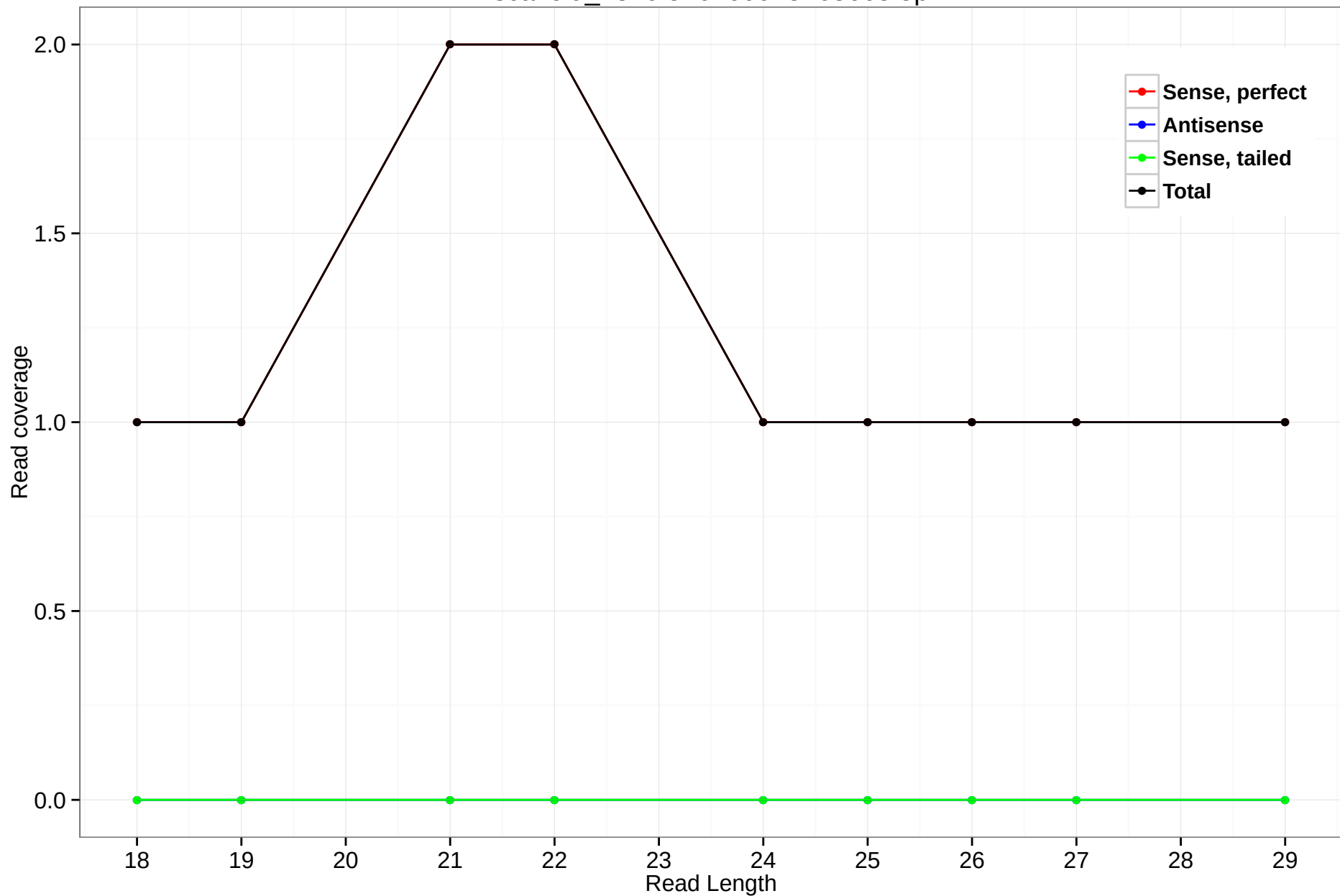
scaffold_4820:5267600-5268663.5p
