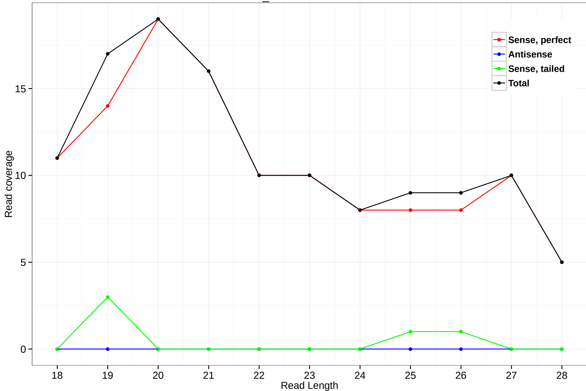
scaffold_4820:5204203-5204360
