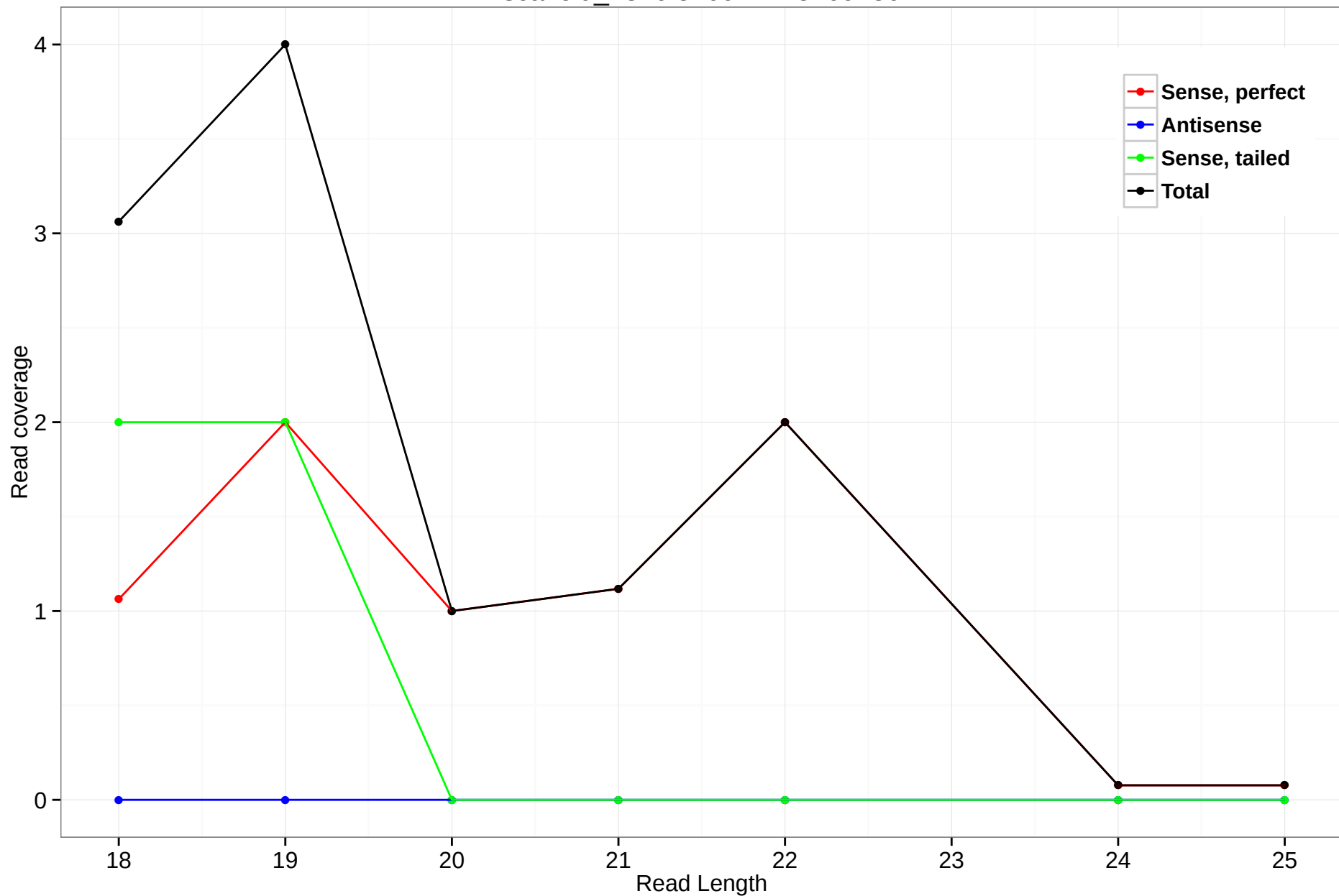
scaffold_4820:5109411-5109736
