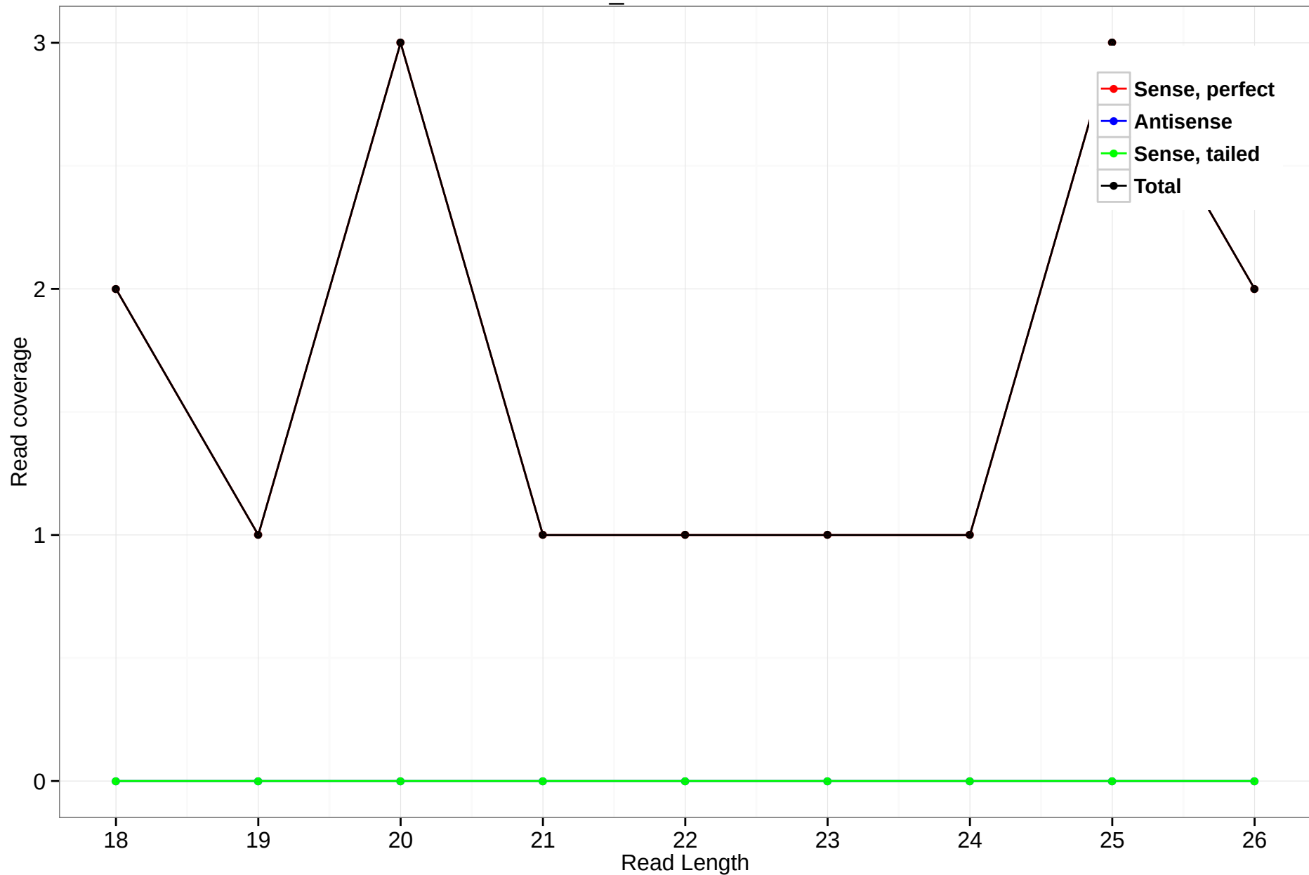
scaffold_4820:49735-49980
