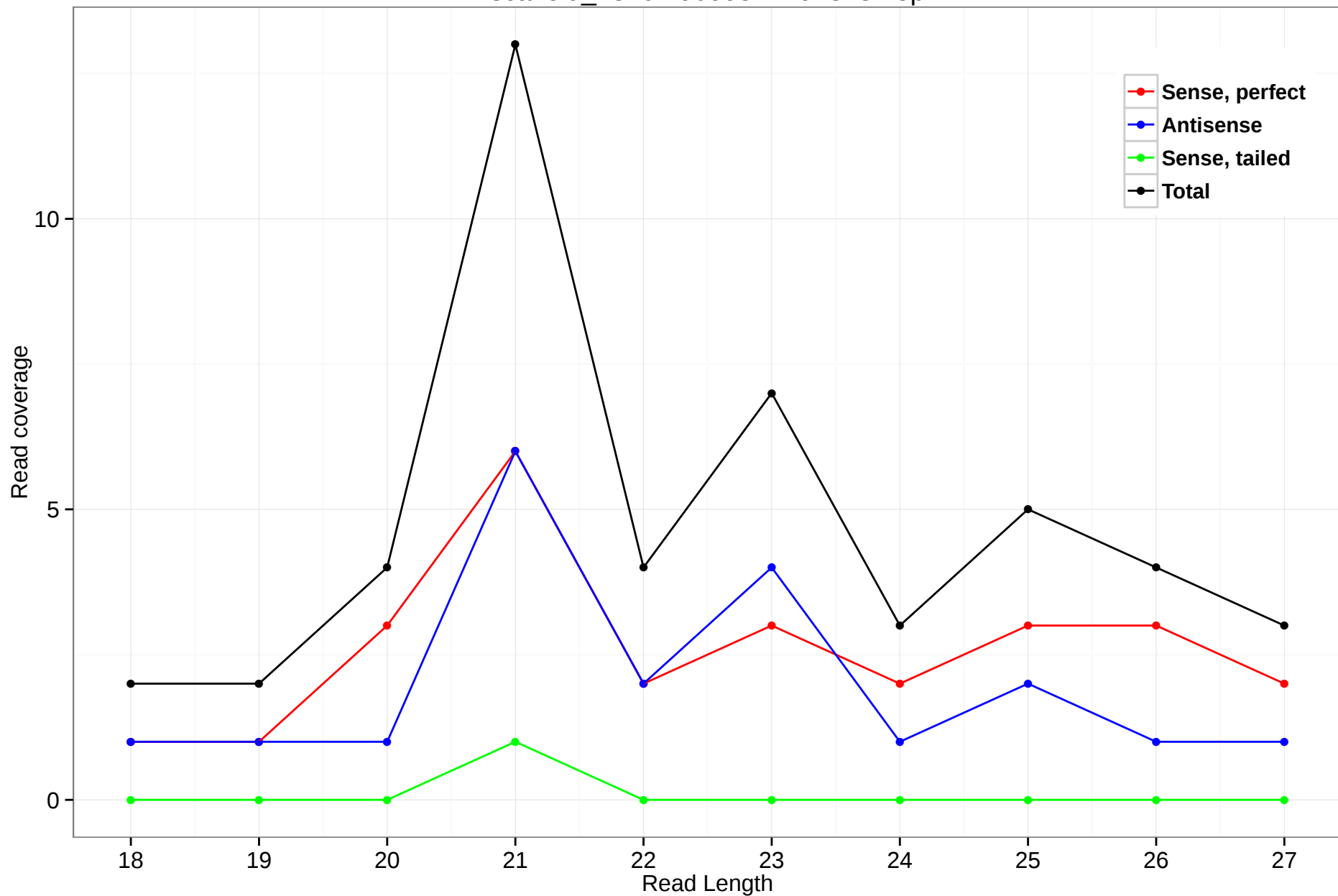
scaffold_4820:4909951-4913232.5p
