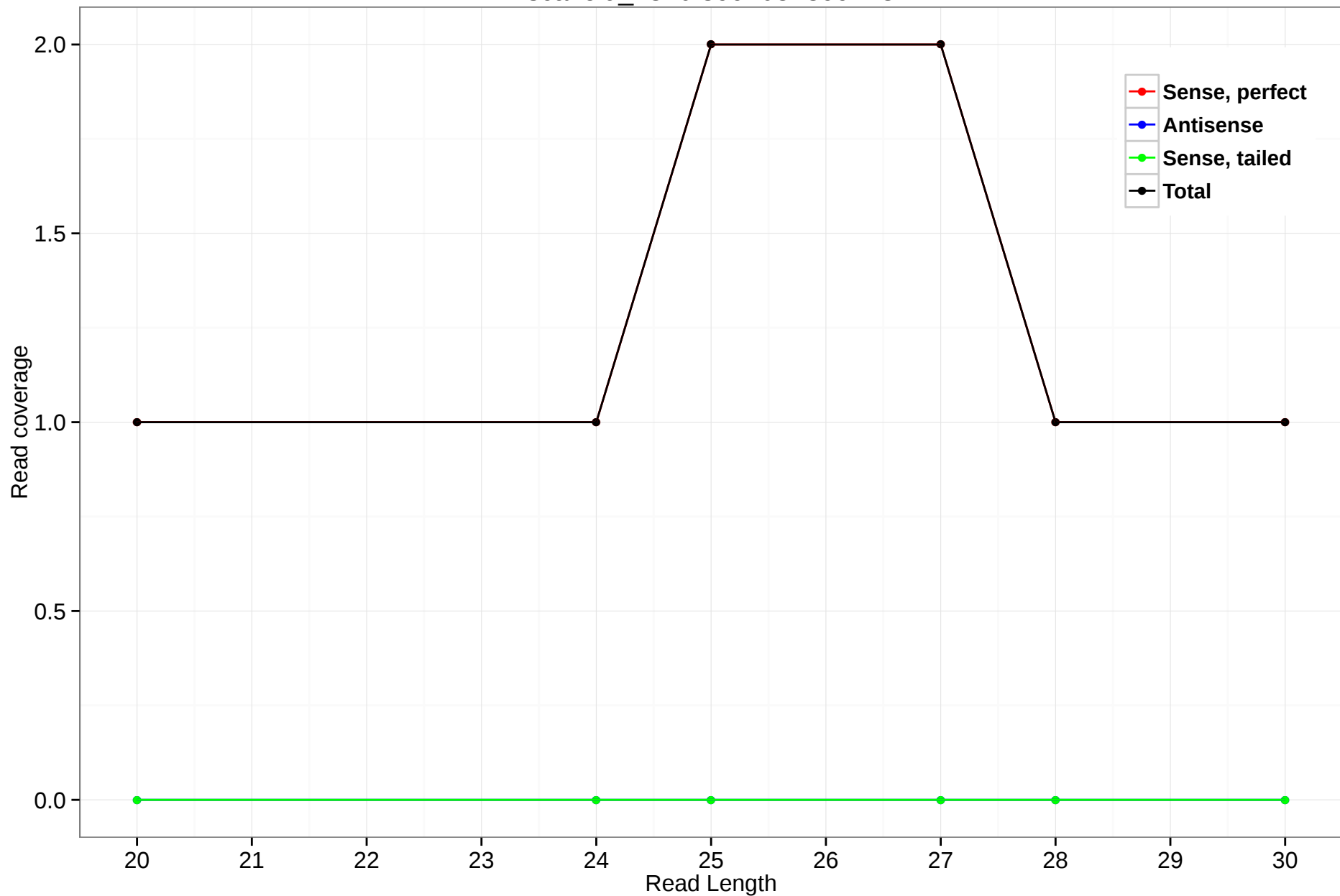
scaffold_4820:399208-399423
