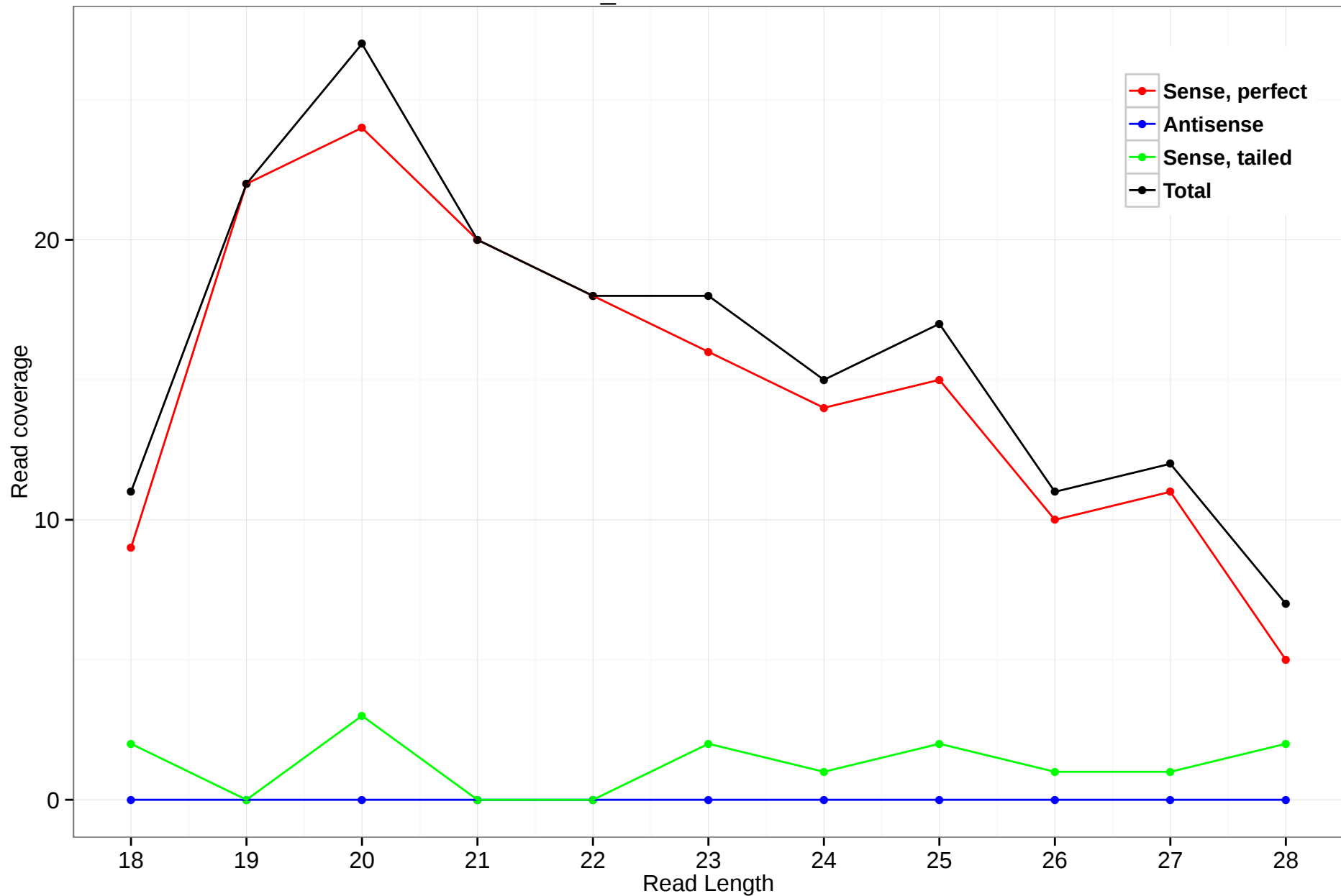
scaffold_4820:3604466-3604863
