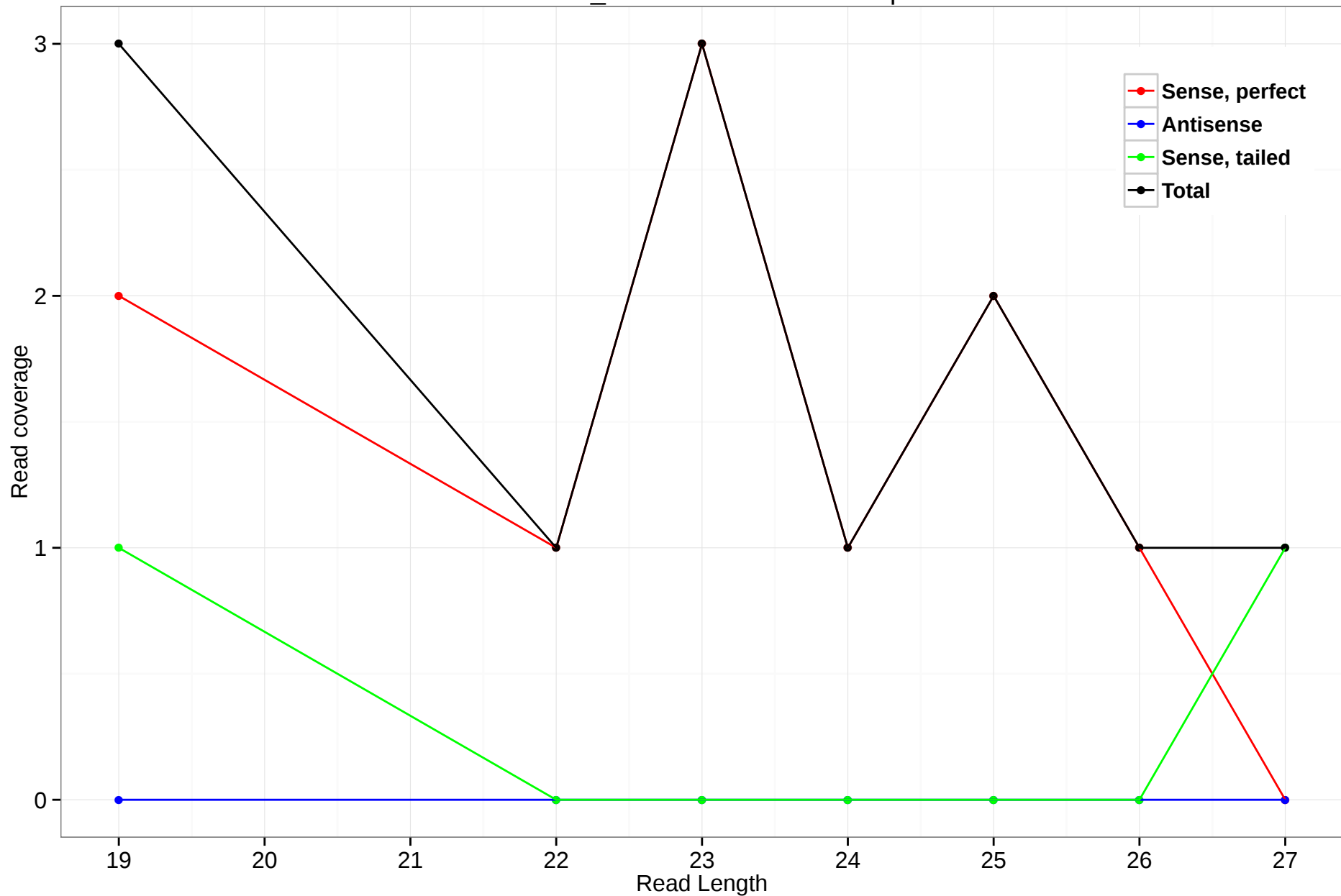
scaffold_4820:355411-356803.5p
