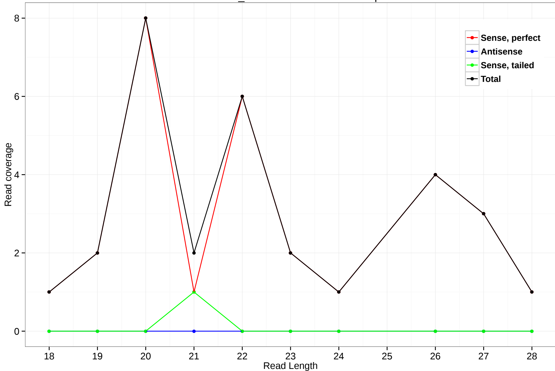
scaffold_4820:3078932-3079664.5p
