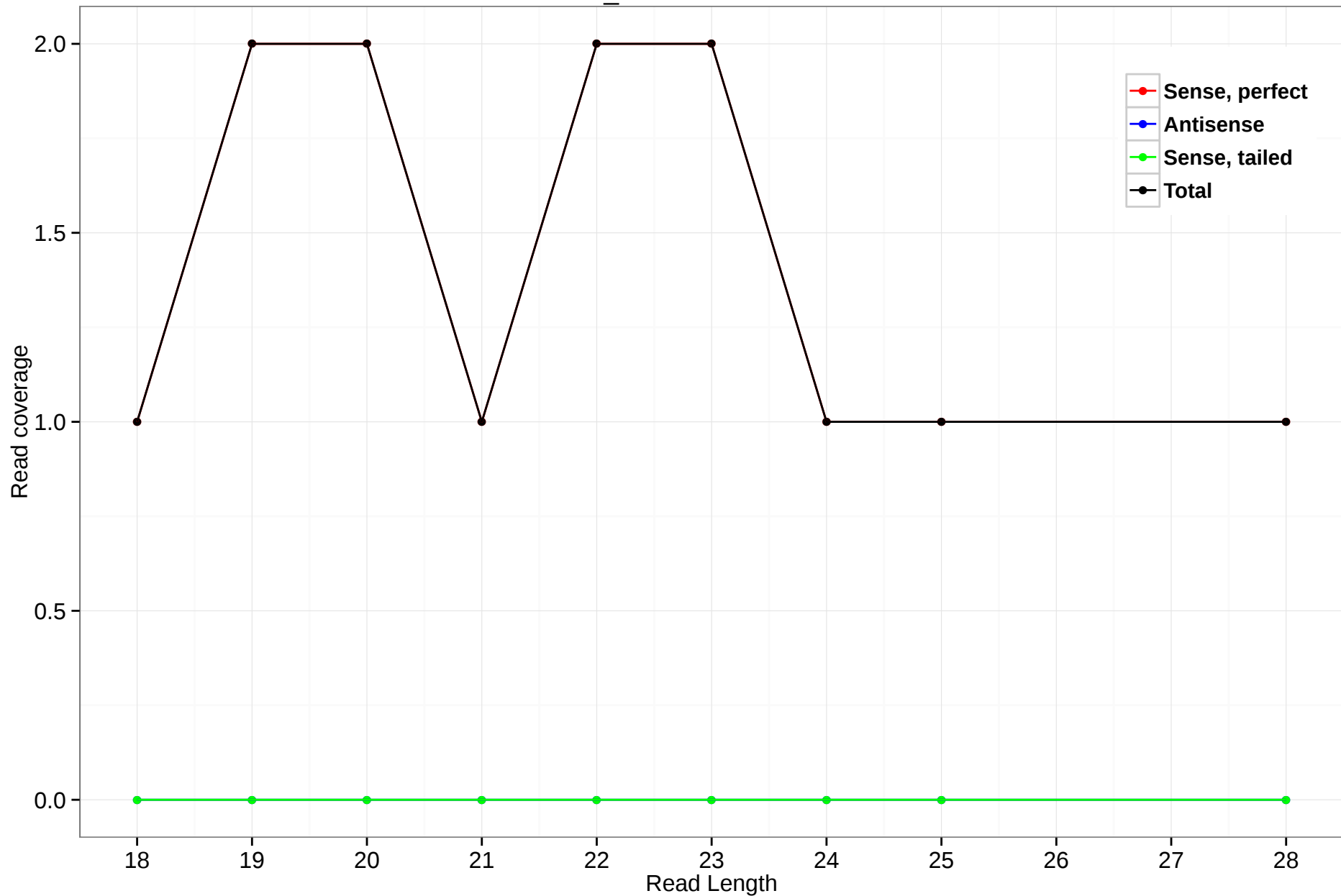
scaffold_4820:2879033-2879204
