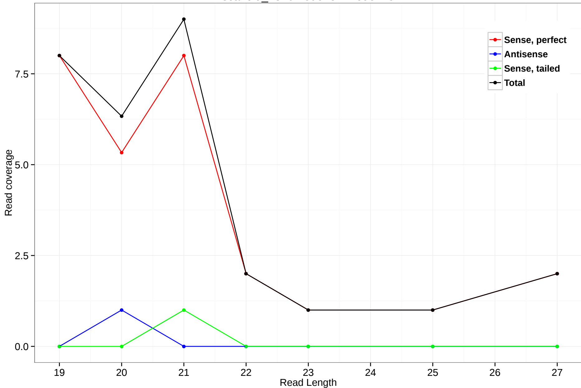
scaffold_4820:2696137-2696429
