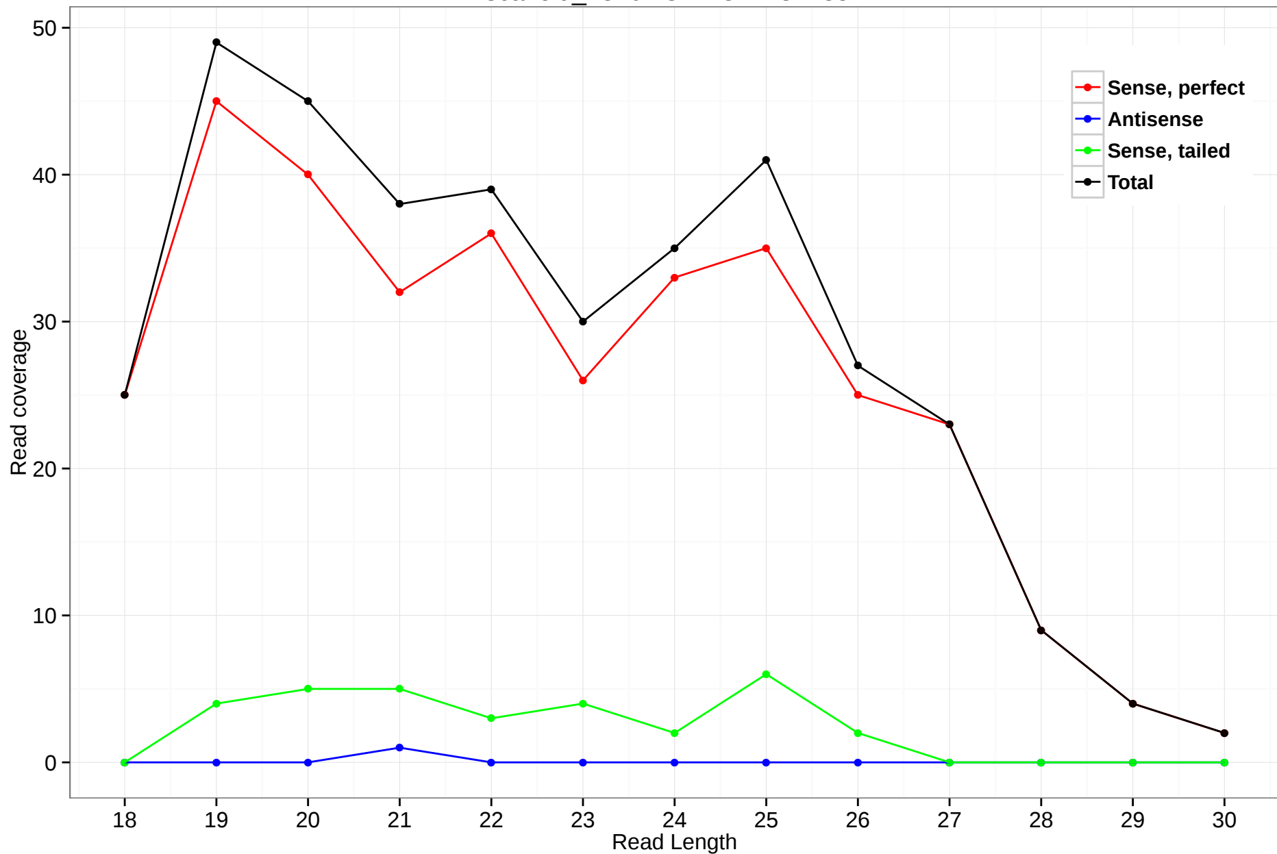
scaffold_4820:2312281-2312852
