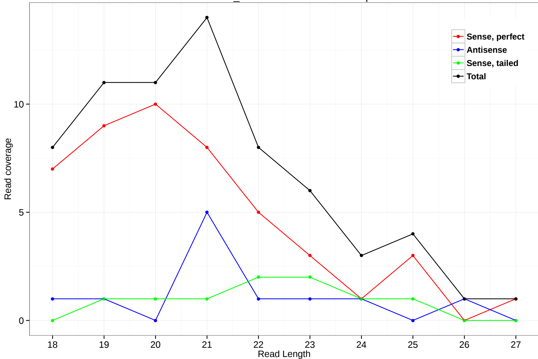
scaffold_4820:2273893-2276026.3p
